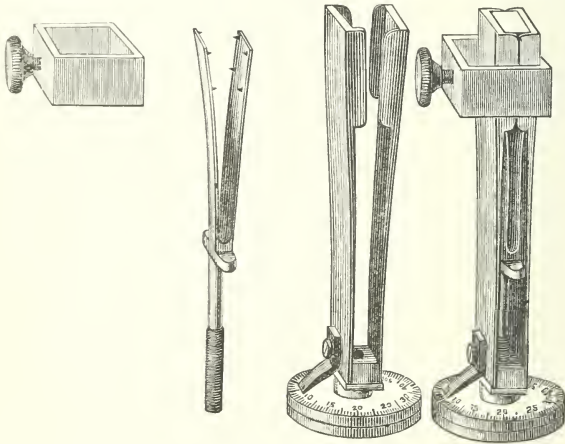
BRAATZ'S HAND-MICROTOME.
