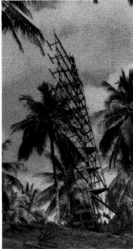
The SCR-270 radar had ten degrees of tilt designed into its frame. Master Tech. Sgt. Dermott H. McDonnell used this feature to advantage in the defense of Guadalcanal.
