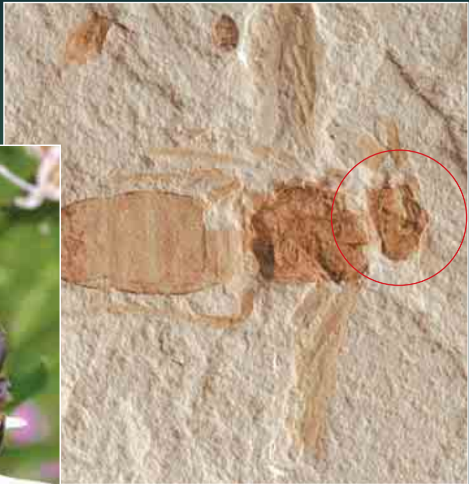
A 48- to 37-million-year-old fossil wasp
