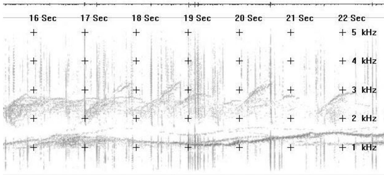
Spectrogram of waveling-tone emissions taped in northern Alberta by Stephen McGreevy on 02 June 1996 via WR-4b
