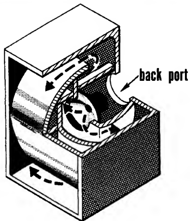
Double-Folded Horn
