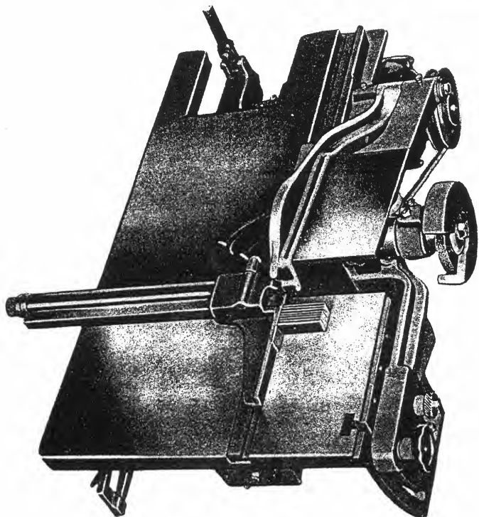
Maximum safety is essential to high-speed production. Saw and emery wheel are almost completely enclosed by guards. Positive work holder permits sawing of slugs as little as 9 points in length. Slugs of 9 points or larger may be trimmed lengthways.
