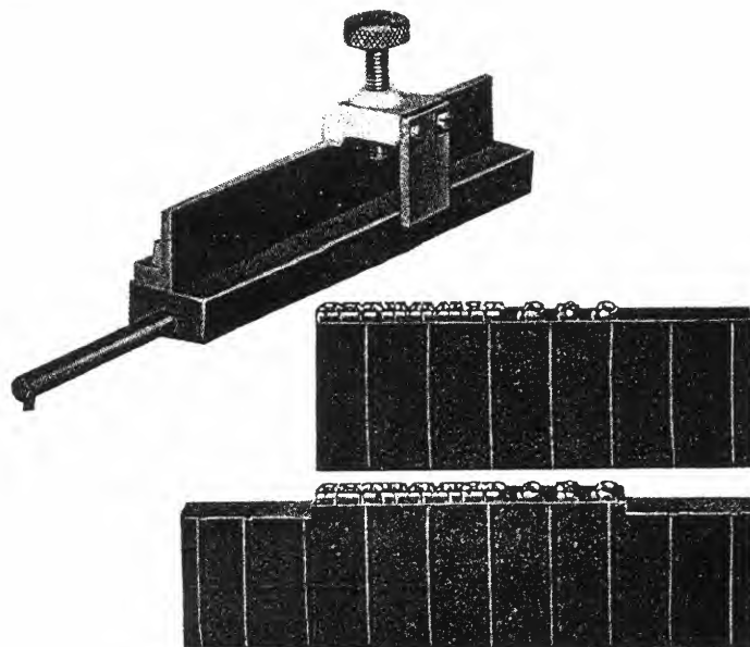
The C&G Low Slug attachment aligns and holds slugs for cutting down high shoulders on short or centered lines. The illustration above shows the attachment, and slugs before and after sawing. Attachment fits in regular vise channel. It operates simply and easily.
