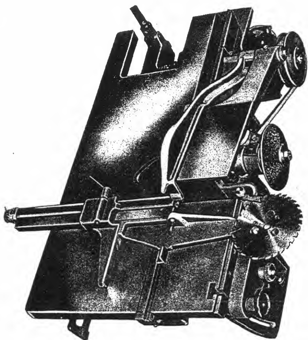
Universal Saw Blade Assembly includes a special Saw Grinding Attachment and Emery Wheel. Universal blades are made of high speed steel for cutting all composing room materials. With the C&G Saw Grinding Attachment the Universal blade may be sharpened in 3 minutes.
