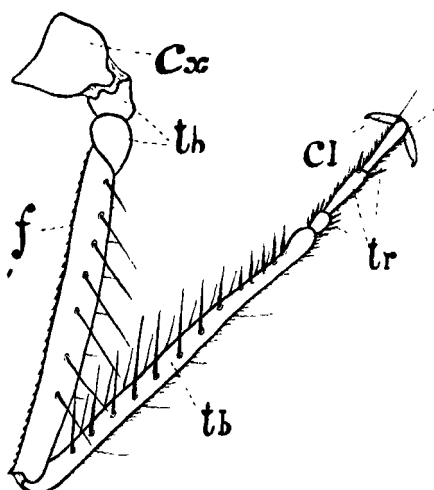
Fig. 4.—Leg of a Zygopterous dragonfly.
