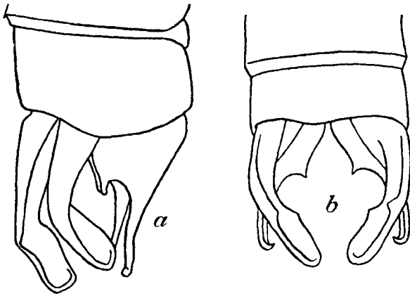
Fig. 60.—Anal appendages of Ceylonosticta hilaris (Selys) male. a. Right lateral view. b. Dorsal view.
