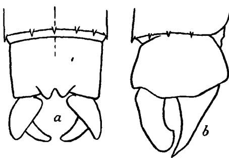
Fig. 176.—Anal appendages of Mortonagrion varralli Fras., male. a. Dorsal view. b. Right lateral view.
