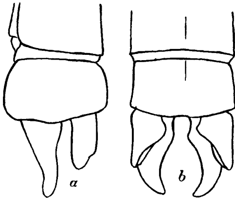
Fig. 85.—Anal appendages of Platycnemis latipes dealbata Solys, male. a. Left lateral view. b. Dorsal view.
