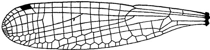
Fig. 179.—Hind-wing of Onychargia atrocyana Selys, male.
