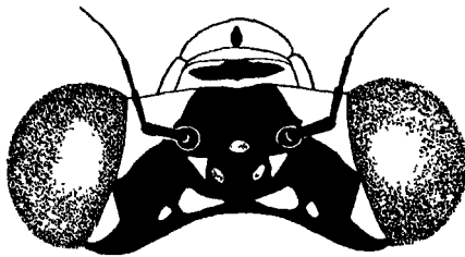
Fig. 91.—Head of Coperia annulata (Selys), male.
