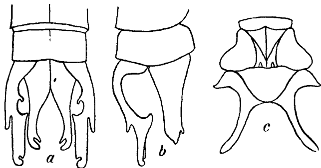
Fig. 50.—Anal appendages and prothorax of Protostictia antelopoides Fras.
