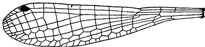
Fig. 150.—Hind-wing of Ischnura senegalensis (Ramb.), male.
