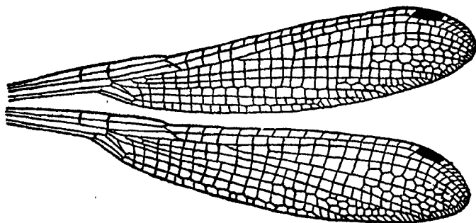
Fig. 6.—Wings of Megalestes major Selys, male.
