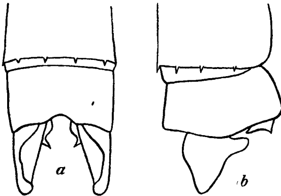
Fig. 164.—Anal appendages of Agriocnemis lacteola Selys, male. a. Dorsal view. b. Right lateral view.
