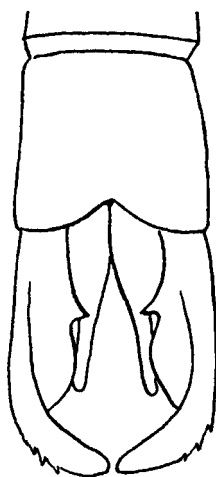
Fig. 19.—Dorsal view of anal appendages of Lestes patricia Fras., male.
