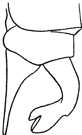
Fig. 55.—Left lateral view of anal appendages of Protosticta uncata Fras.
