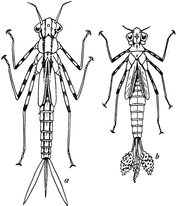
Fig. 1.—Larvæ of:—a. Agrine ( Neurobasis chinensis ); b. Cœnagriine ( Cooper marginipes ).
