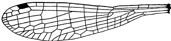
Fig. 163.—Hind-wing of Agriocnemis pygmaea (Ramb.), male.
