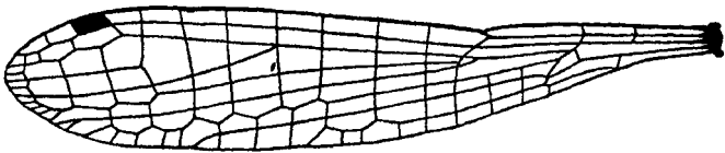
Fig. 144.—Hind-wing of Aciagrion hisopa Selys, male.
