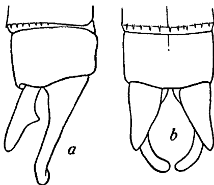
Fig. 73.—Anal appendages of Cæliccia renifera (Selys), male. a. Right lateral view. b. Dorsal view.
