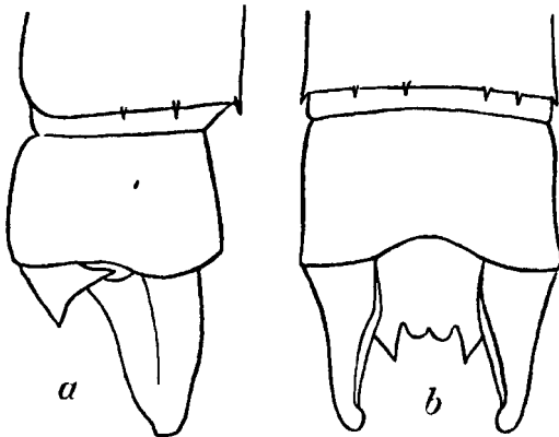
Fig. 167.—Anal appendages of Agriocnemis clauseni Fras., male. a. Left lateral view. b. Dorsal view.
