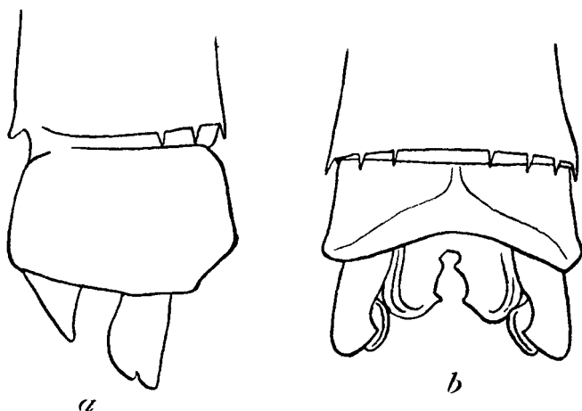
Fig. 131.—Anal appendages of Archibasis mimetes praecleara (Fras.), male. a. Left lateral view. b. Dorsal view.
