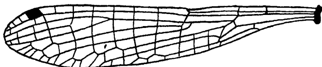
Fig. 158.—Hind-wing of Rhodischnura nursei (Mort.), male.
