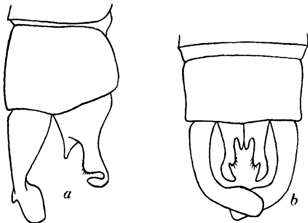
Fig. 58.—Anal appendages of Platysticta apicalis Kirby, male. a. Right lateral view. b. Dorsal view.
