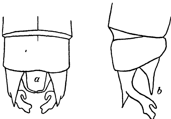
Fig. 51.—Anal appendages of Protosticta sanguinostigma Fras., male. a. Dorsal view. b. Right lateral view.
