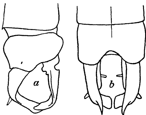
Fig. 69.—Anal appendages of Drepanosticta viridis Fras., male. . a. Right lateral view. b. Dorsal view.
