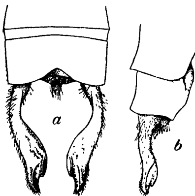
Fig. 40.—Anal appendages of Burmargiolestes melanothorax (Selys). a. Dorsal view. b. Right lateral view.
