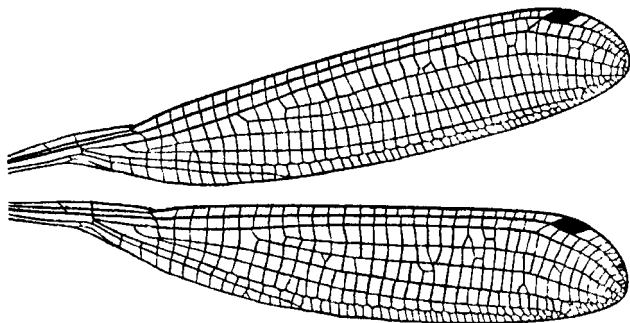
Fig. 115.—Wings of Phylloneura westermanni (Solys), male.
