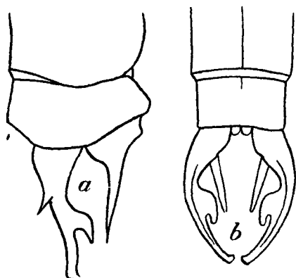
Fig. 52.—Anal appendages of Protosticta mortoni Fras., male. a. Right lateral view. b. Dorsal view.
