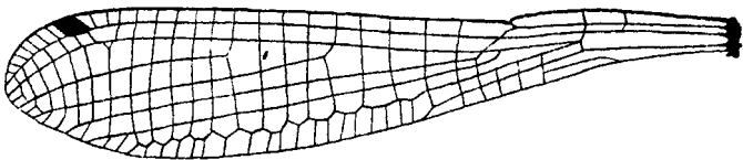
Fig. 98.—Wing of Disparoneura atkinsoni Selys, male.
