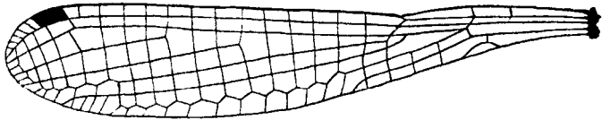
Fig. 96.—Wing of Caconeura verticalis annandalei Fras., male.
