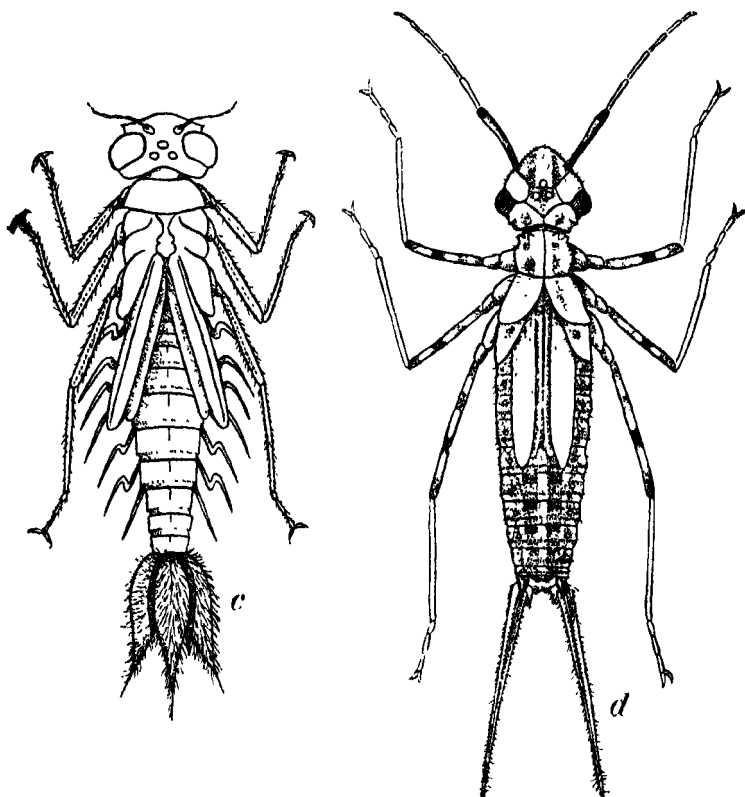
Fig. 1.—Larvæ of :—c. Epallaginine ( Indophaea fraseri ); d. Libellaginine ( Libellago lineata indica ).
