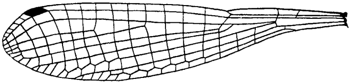
Fig. 86.—Wing of Copera marginipes (Ramb.), male.
