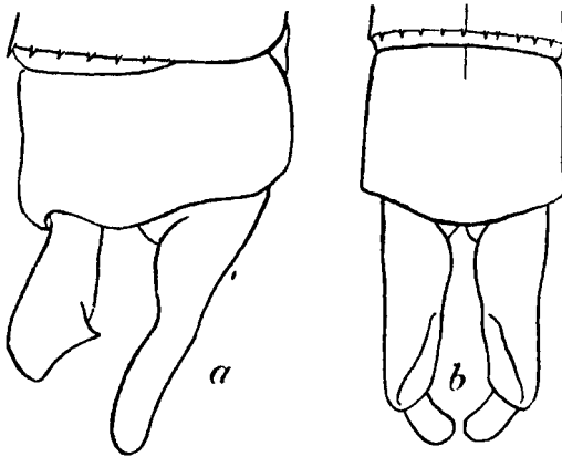
Fig. 76.—Anal appendages of Cœlaccia poungyi Fras., male. a. Right lateral view. b. Dorsal view.
