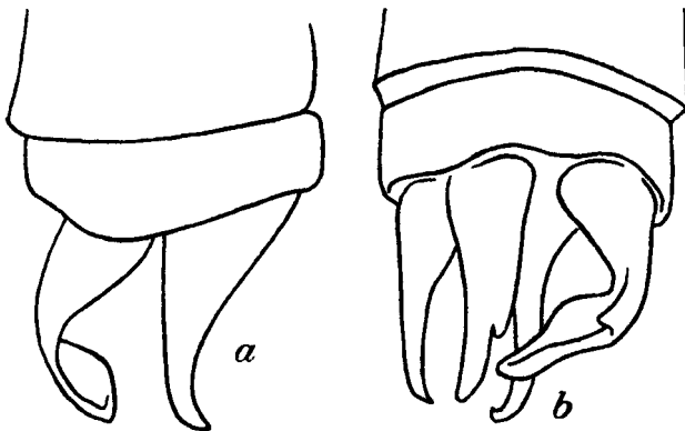
Fig. 68.—Anal appendages of Drepanosticta carmichaeli Laid. a. Right lateral view. b. Dorsal view.
