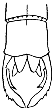
Fig. 36.—Dorsal view of anal appendages of Indolestes indica Fras., male.
