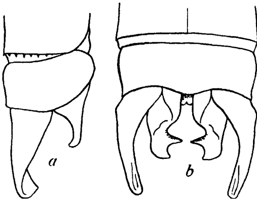
Fig. 63.—Anal appendages of Ceylonosticta digna (Selys). a. Right lateral view. b. Dorsal view.
