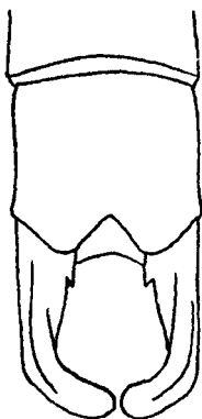
Fig. 17.—Dorsal view of anal appendages of Lestes angularis Fras., male.
