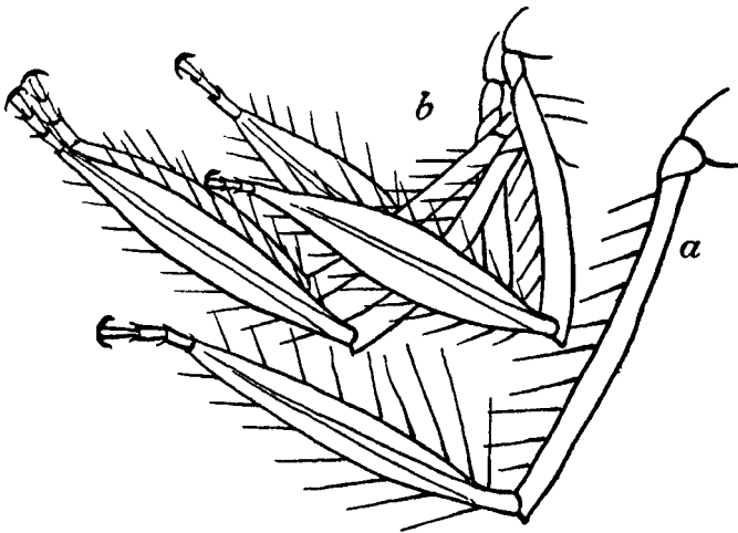
Fig. 94.—Legs of :— a. Copera annulata (Selys), male ; b. Copera superplatypes Fras., male, showing the dilated tibiae of the two hind pairs of legs.
