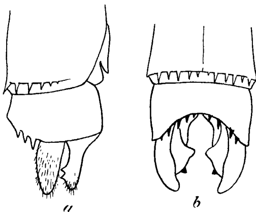
Fig. 125.—Anal appendages of Pseudagrion rubriceps Selys, male. a. Right lateral view. b. Dorsal view.
