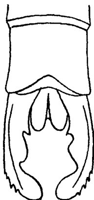
Fig. 15.—Dorsal view of anal appendages of Lestes elata Hagen, male.
