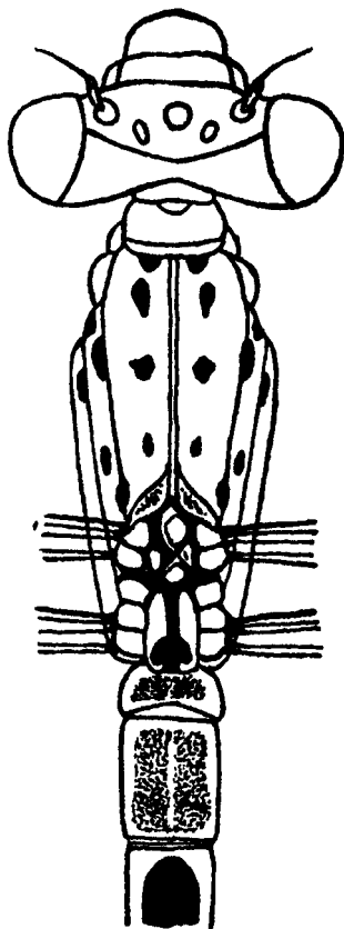
Fig. 25.—Head and thorax of Platylestes platystyla (Ramb.), showing markings.
