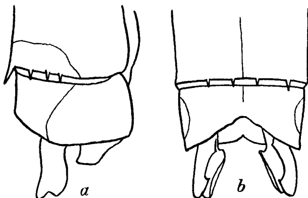
Fig. 126.—Anal appendages of Pseudagrion williamsoni Fras., male. a. Right lateral view. b. Dorsal view.
