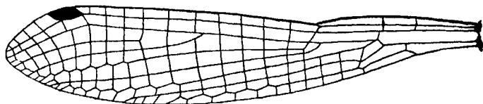
Fig. 173.—Hind-wing of Argiocnemis rubescens Selys, male.
