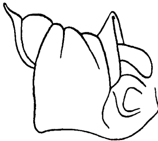
Fig. 66.—Prothorax of Ceylonosticta walli Fras., female. Posterior lobe to the left.
