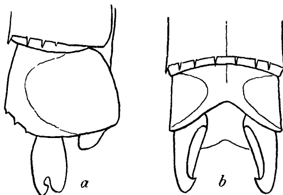
Fig. 124.—Anal appendages of Pseudagrion laidlawi Fras., male. a. Right lateral view. b. Dorsal view.
