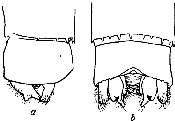
Fig. 136.—Anal appendages of Ceriagrion prætermisum Lieft., male. a. Left lateral view. b. Dorsal view.
