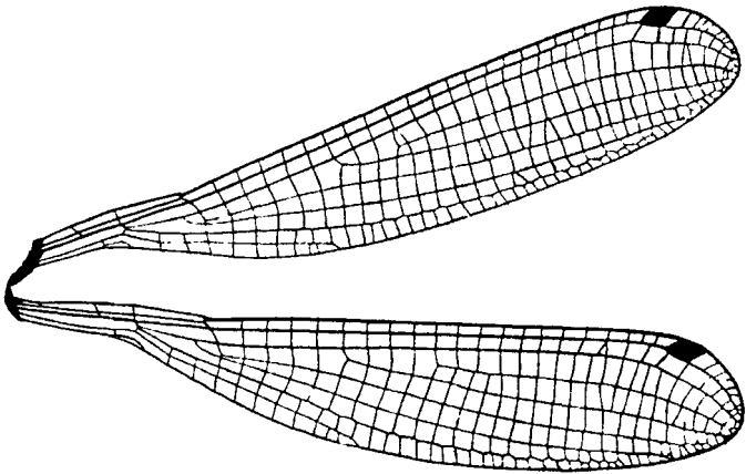
Fig. 104.—Wings of Indoneura ramburi Fras., male.
