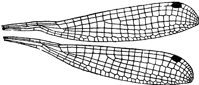
Fig. 47.—Wings of Protosticta himalaica Laid., male.
