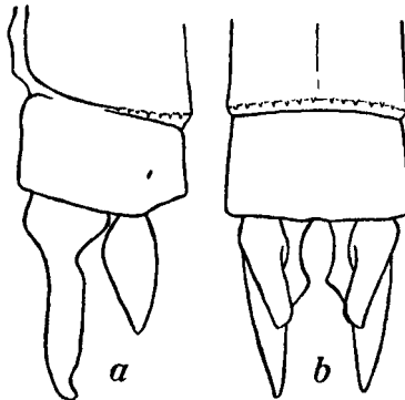
Fig. 90.—Anal appendages of Copera assamensis Laid., male. a. Left lateral view. b. Dorsal view.
