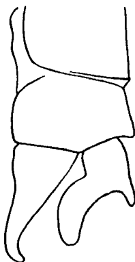
Fig. 110.—Anal appendages of Melanoneura bilineata Fras., male, viewed from the left.
