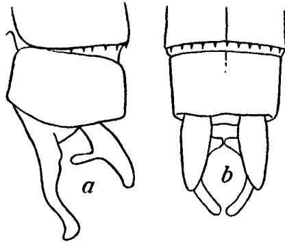
Fig. 80. -Anal appendages of Calicnemis miles Laid., male. a. Left lateral view. b. Dorsal view.
