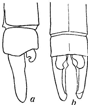
Fig. 87.—Anal appendages of Copera marginipes (Ramb.), male. a. Left lateral view. b. Dorsal view.
