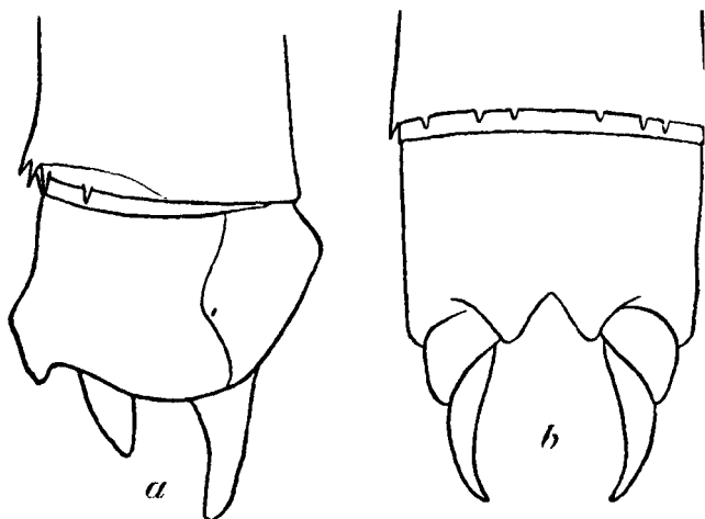
Fig. 154.—Anal appendages of Ischnura inarmata Calv., male. a. Right lateral view. b. Dorsal view.
