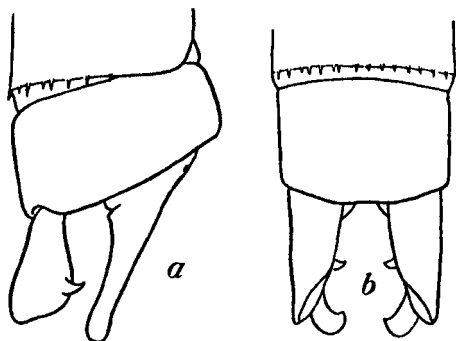
Fig. 77.—Anal appendages of Cœliccia chromothorax (Selys), male. a. Right lateral view. b. Dorsal view.
