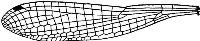
Fig. 160.—Hind-wing of Enallagma cyathigerum Charp., male.
