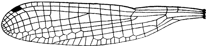
Fig. 84.—Wing of Platycnemis latipes dealbata Selys, male.
