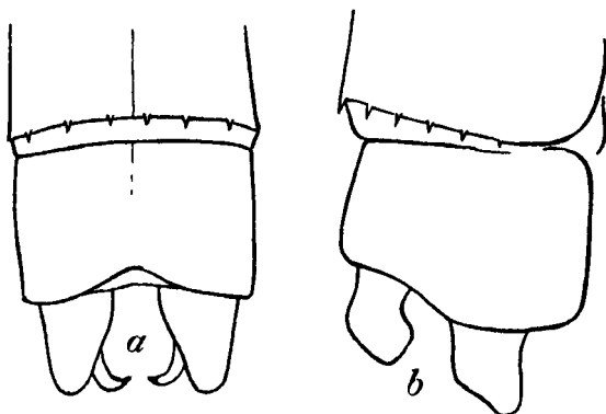
Fig. 171.—Anal appendages of Agriocnemis pygmaea (Ramb.), male. a. Dorsal view. b. Right lateral view.
