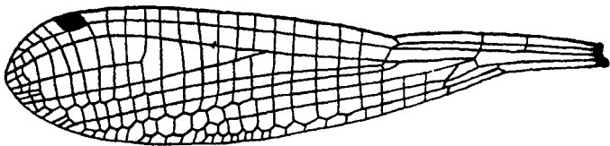
Fig. 142.—Hind-wing of Himalagrion exclamatoris Fras., male.
