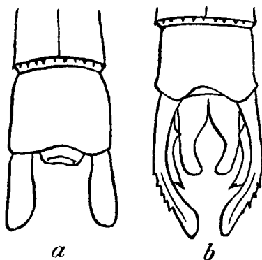
Fig. 26.—Anal appendages of Platylestes platystyla (Ramb.). a. Dorsum of female. b. Dorsal view of male.
