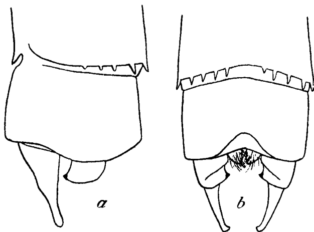
Fig. 140.—Anal appendages of Ceratagrion cerinorubellum (Brauer), male. a. Left lateral view. b. Dorsal view.
