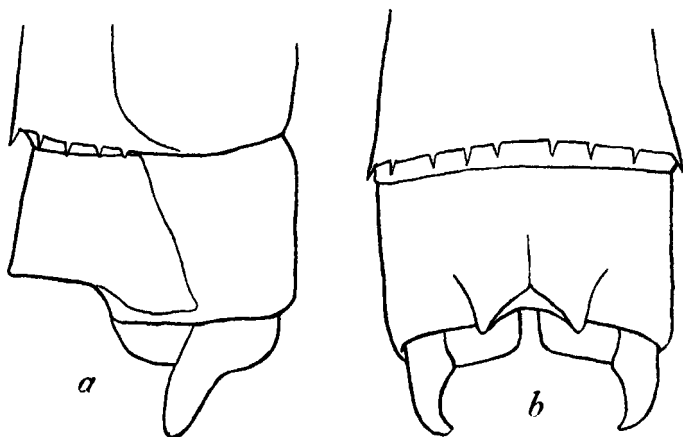
Fig. 151.—Anal appendages of Ischnura senegalensis (Ramb.), male. a. Right lateral view. b. Dorsal view.
