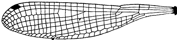
Fig. 79.—Wing of Calicnemis miniata Selys, male.
