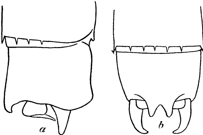
Fig. 157.—Anal appendages of Ischnura annandalei Laid., male. a. Right lateral view. b. Dorsal view.
