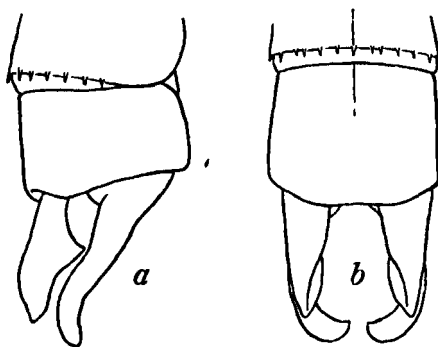
Fig. 74.—Anal appendages of Caeliccia didyma (Selys), male. a. Right lateral view. b. Dorsal view.
