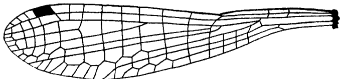
FIG. 175.—Hind-wing of Mortonagrion varralli Fras., male.
