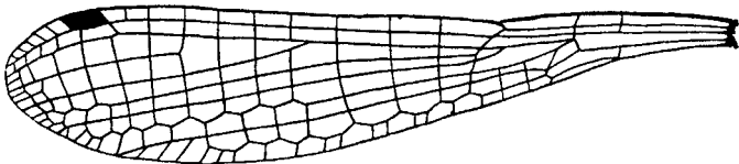
Fig. 117.—Hind-wing of Pseudagrion spencei Fras., male.
