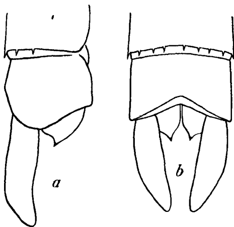
Fig. 168.—Anal appendages of Agriocnemis splendidissima Laid., male, a. Right lateral view. b. Dorsal view.
