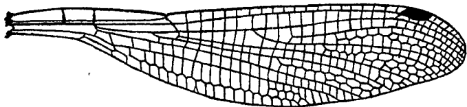
Fig. 44.—Hind-wing of Mesopodagrion tibetanum MacL., male.
