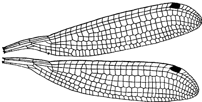
Fig. 56.—Wings of Platysticta deccanensis Laid., male.
