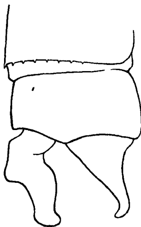
Fig. 116.—Anal appendages of Phylloneura westermanni (Selys), male, viewed from the right side.
