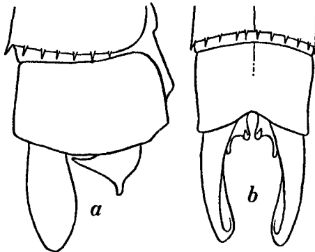
Fig. 174.—Anal appendages of Argiocnemis rubescens Selys, male. a. Right lateral view. b. Dorsal view.
