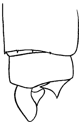
Fig. 165.—Anal appendages of Agriocnemis nana (Laid.), male, right side.
