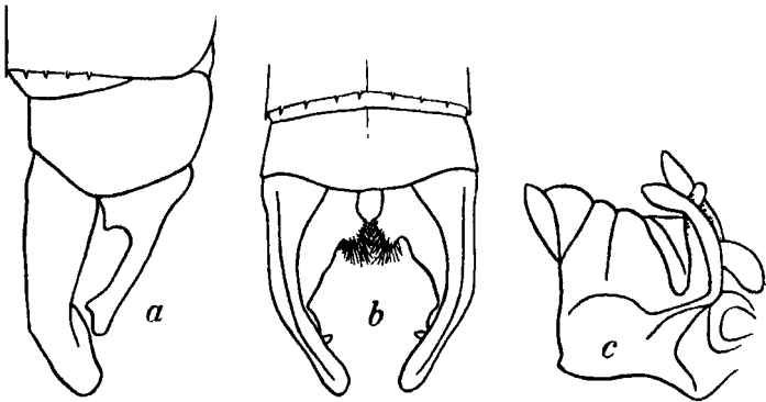
Fig. 62.—Anal appendages and prothorax of Ceylonosticta tropica (Selys).
