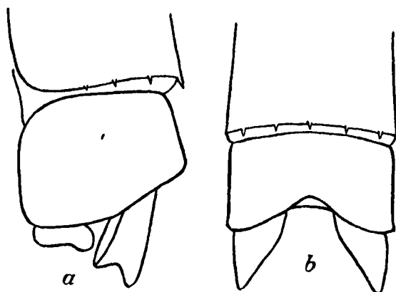
Fig. 146.—Anal appendages of Acia grion olympicum Laid., male. a. Left lateral view. b. Dorsal view.
