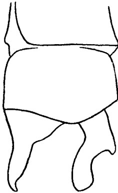
Fig. 114.—Anal appendages of Esmé longistyla Fras., male, viewed from the left.
