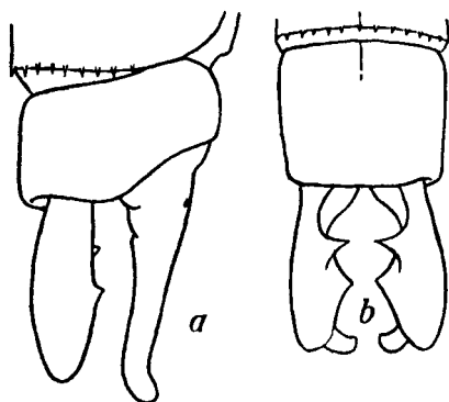
Fig. 78.—Anal appendages of Caliccia fraseri Laid., male. a. Right lateral view. b. Dorsal view.
