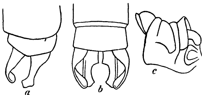
Fig. 64.—Anal appendages and prothorax of Ceylonostieta nietneri Fras., male.
