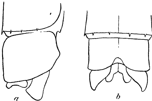
Fig. 149.—Anal appendages of Aciagrion pallidum Selys, male. a. Right lateral view. b. Dorsal view.
