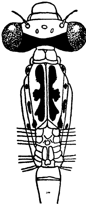
Fig. 11.—Head and thorax of Lestes praeorsus Selys, showing markings.
