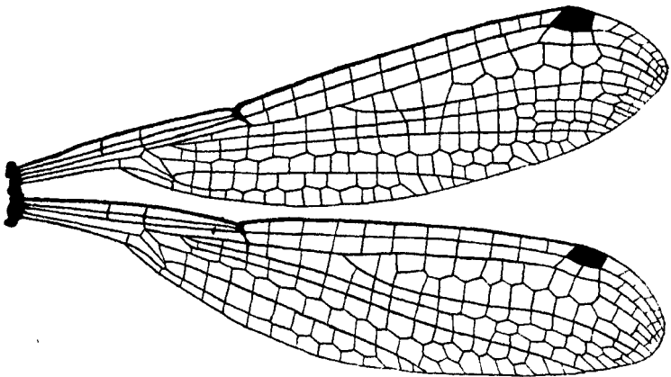
Fig. 24.—Wings of Platylestes platystyla (Ramb.), male.
