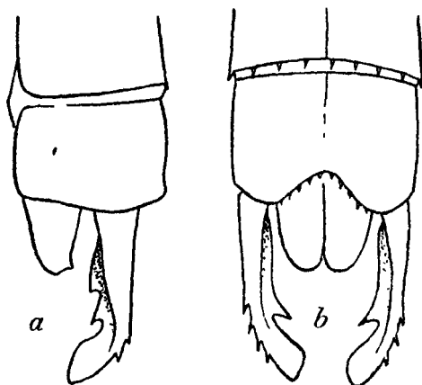
Fig. 29.—Anal appendages of Ceylonolestes divisa (Hagen-Selys), male. a. Left lateral view. b. Dorsal view.
