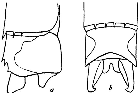
Fig. 120.—Anal appendages of Pseudagrion malabaricum Fras., male. a. Right lateral view. b. Dorsal view.
