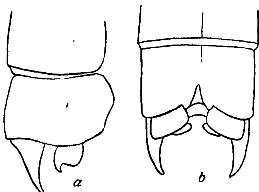
Fig. 161.—Anal appendages of Enallagma cyathigerum Charp., male. a. Left lateral view. b. Dorsal view.
