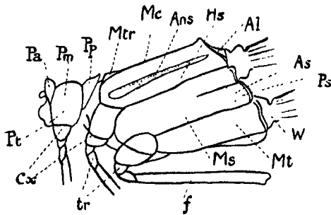
Fig. 3.—Prothorax and thorax of a Zygopterous dragonfly.
