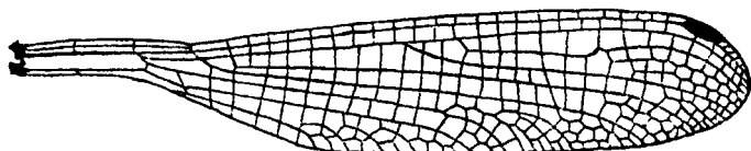
Fig. 39.—Fore-wing of Burmargiolestes melanothorax (Selys), male.
