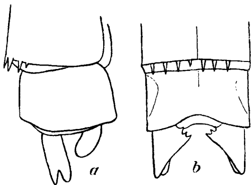
Fig. 118.—Anal appendages of Pseudagrion microcephalum (Ramb.), male. a . Right lateral view. b . Dorsal view.
