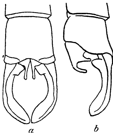
Fig. 8.—Anal appendages of Megalstes irma Fraser, male. a. Dorsal view. b. Left lateral view.
