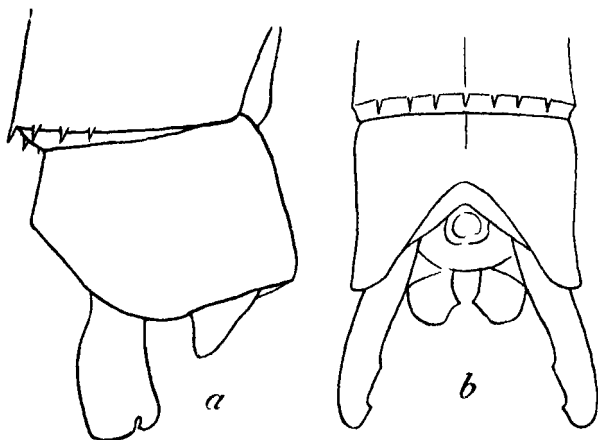
Fig. 128.—Anal appendages of Pseudagrion pruinosum Selys, male. a. Right lateral view. b. Dorsal view.
