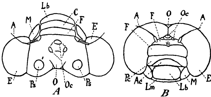
Fig. 2.—A. Head of a Zygopterous dragonfly seen from above.
