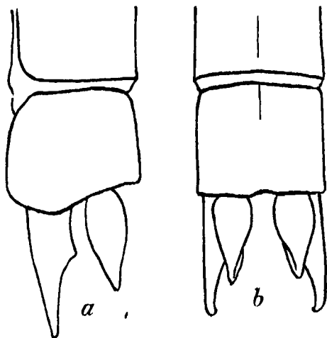
Fig. 95.—Anal appendages of Copera superplatypes Fras., male. a. Left lateral view. b. Dorsal view.
