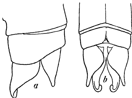
Fig. 97.—Anal appendages of Caconeura verticalis annandalei Fras. a. Left lateral view. b. Dorsal view.
