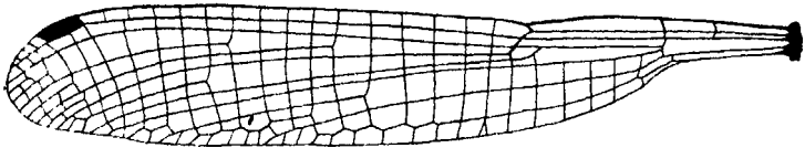
Fig. 41.—Hind-wing of Rhinagrion mima (Karsch), male.
