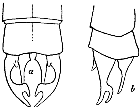
Fig. 48.—Anal appendages of Protosticta graveleyi Laid., male. a. Dorsal view. b. Right lateral view.
