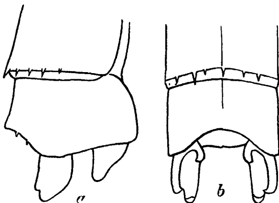
Fig. 127.—Anal appendages of Pseudagrion indicum Fras., male. a. Right lateral view. b. Dorsal view.
