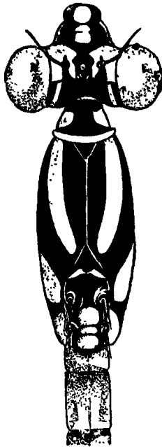
Fig. 42.—Head and thorax of Rhinagrion mimia (Karsch), male, showing markings.
