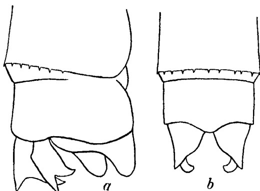
Fig. 103.—Anal appendages of Chloroneura quadrimaculata (Ramb.), male. a. Right lateral view. b. Dorsal view.
