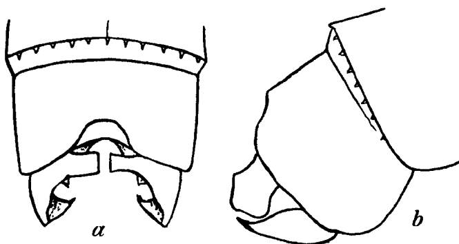
Fig. 162.—Anal appendages of Enallagma parvum Selys, male. a. Dorsal view. b. Right lateral view.
