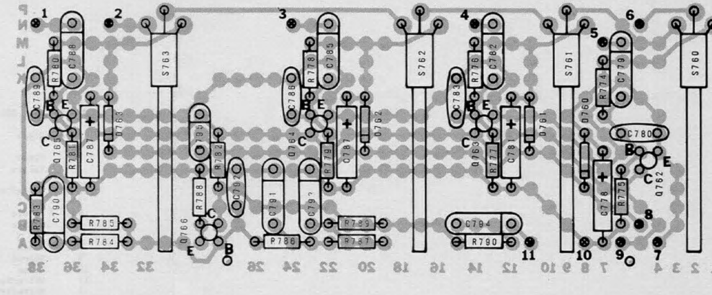
FIGURE 5-6 PEDAL KEYER BOARDS 124-000025, 124-000026, 124-000027, LAYOUT & SCHEMATIC
