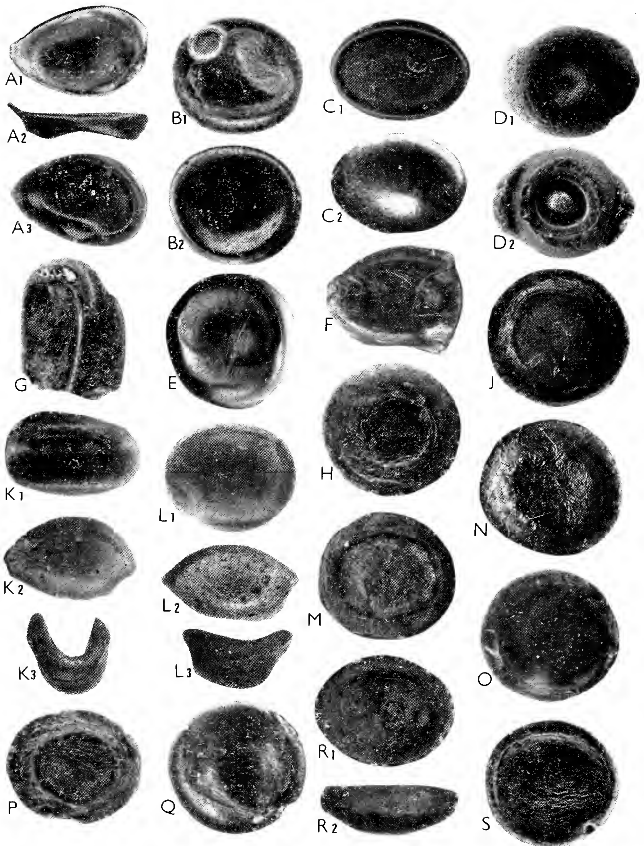
Figure 5.—Australites from Western Australia and Victoria. Illustrations are plan views (i.e. posterior surfaces of flight) unless stated otherwise. For details of specimens numbered 1-42, see Table 1. Scales vary slightly and may be judged by the dimensions given here or in Table 1. A1.—Teardrop bowl, length 13.4 mm, Menangina Station, W.A. (WASM 10 609). A2.—Side elevation of A1 showing frontal collapse. A3.—Anterior surface of A1 showing limitation of collapse by flow ridge. B1.—Broad oval, "tray" type, length 10.9 mm, Menangina Station, W.A. (WASM 10 614). B2.—Anterior surface of B1 showing frontal collapse. C1.—Narrow oval "tray" type, length 9.0 mm, Menangina Station, W.A. (WASM 10 609). C2.—Anterior surface of C1 showing frontal collapse. D1.—Anterior surface of fragment of hollow button, length 11.5 mm, Mt Remarkable Station, W.A. (KJ). Central collapse dimple over bubble cavity. D2.—Posterior view of D1 showing boss resulting from frontal collapse within breached bubble cavity. E.—Anterior surface of frontally collapsed broad oval bowl from Port Campbell, Vic. (NMV E7821). For details see Table 2. For transverse section see Fig. 4-L2. F.—Pine-seed form, length 10.6 mm, Earahedy Station, W.A. (WASM 10 943). Flange broken from left end, overfolded at right end and fused to body which is visible through it. G.—Fragment of elongated "tray" type australite with thickened edge, length 9.0 mm, fold hinge along right-hand edge, i.e. right hand half of visible surface is anterior surface of flight. Mt Remarkable Station, W.A. (KJ). H.—No. 2. J.—No. 3. K1 to K3.—Plan, side and end elevations of No. 6. L1 to L3.—Plan, side and end elevations of No. 8. M.—No. 10. N.—No. 12. O.—No. 13. P.—No. 14. Q.—No. 15. R1 and R2.—Plan and side elevations of No. 16. S.—No. 18.
