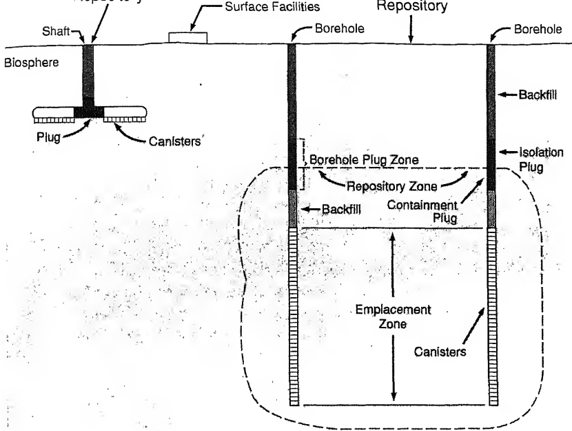
FIGURE 6-3 Deep borehole disposal
