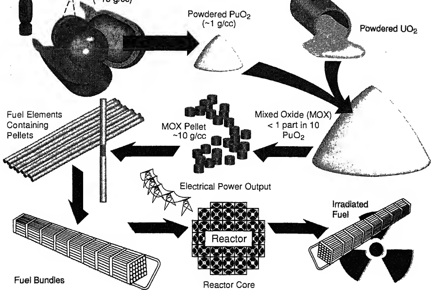
FIGURE 6-2 Steps in the spent fuel option
