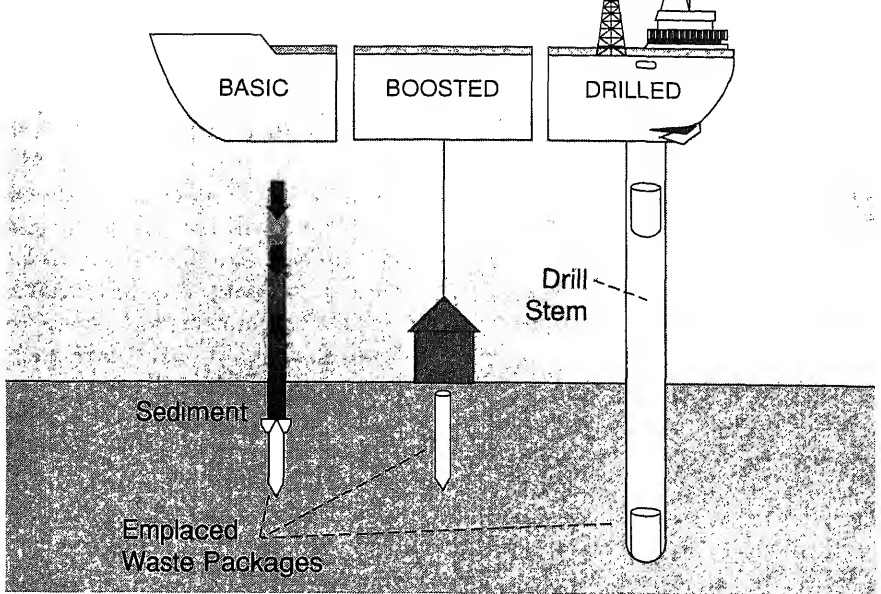
FIGURE 6-4 Sub-seabed disposal
