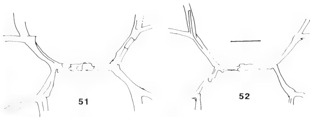
Figures 51, 52. Dichograptus expansus Harris and Thomas, part and counterpart of funicular region of P73512 from Whittings Quarry. Scalebar 1 mm.
