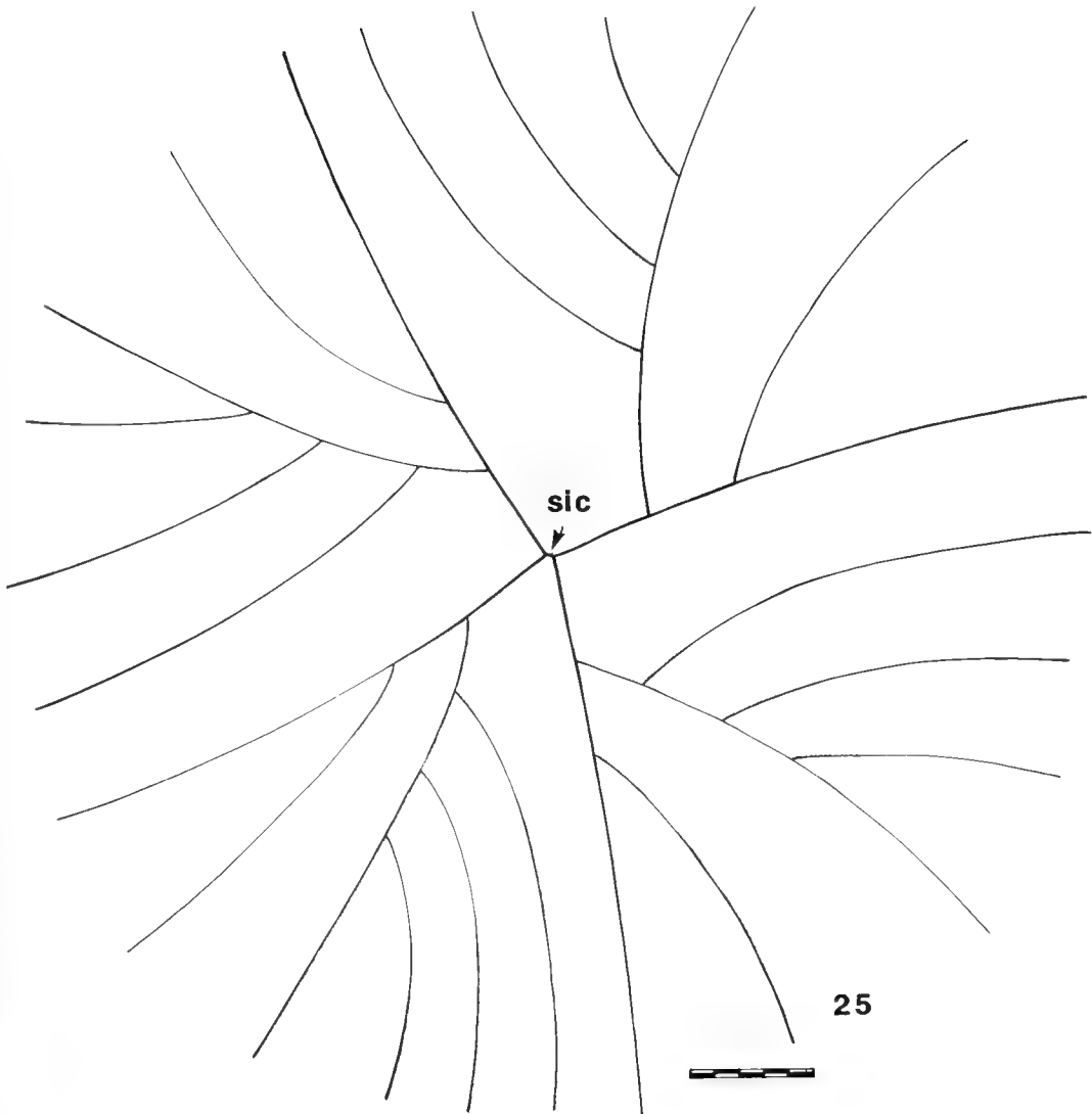
Figure 25. Trochograptus indignis , reconstruction of rhabdosomes based upon lectotype, P83291, probably in plan view of life position. sic = position of sicula and funicle. Scalebar 50 mm.
