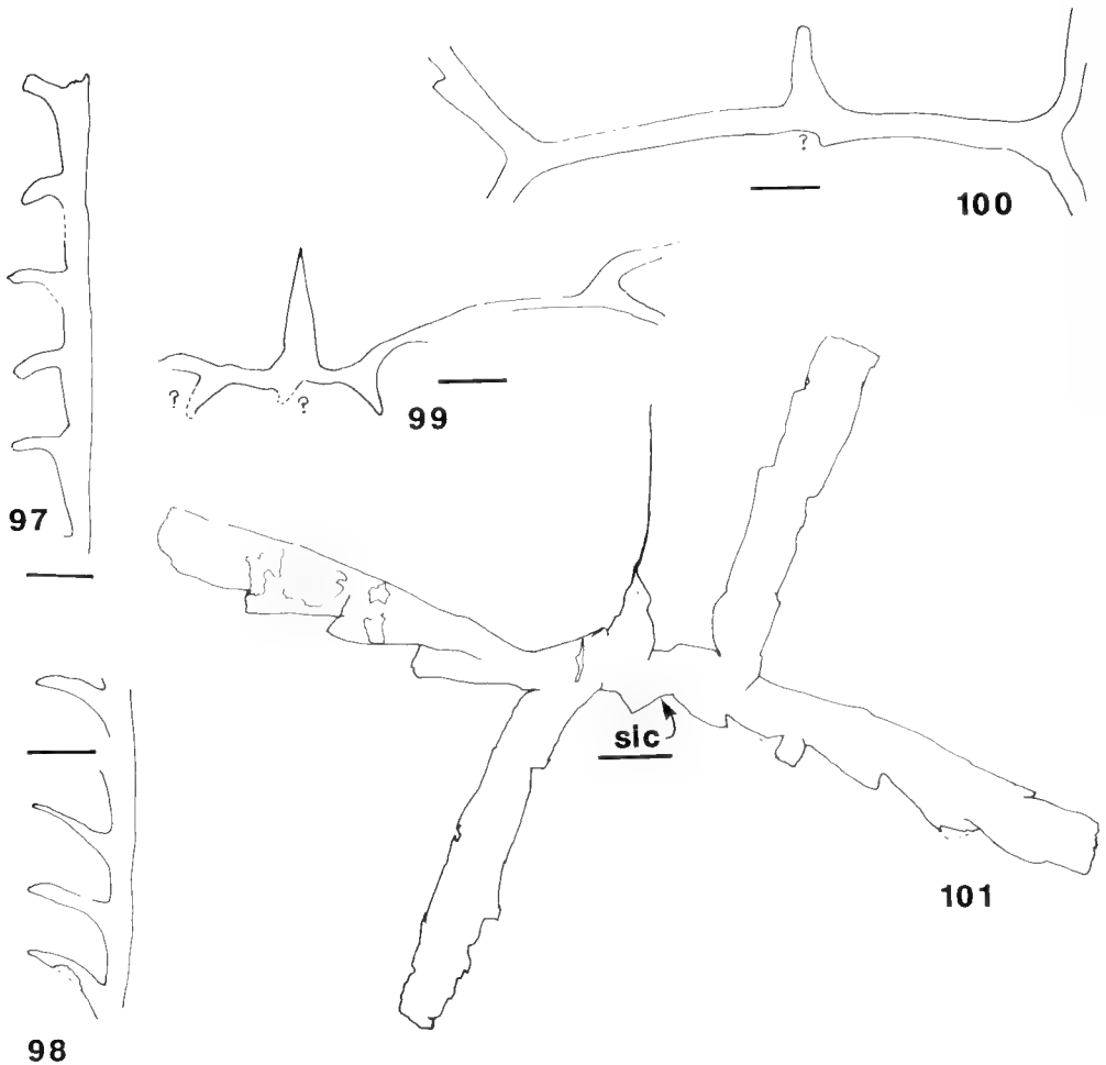
Figures 97, 98. Tetraraptus (? Tetraraptus ) chapmani Keble and Harris: 97, thecae on 2nd order stipe of holotype P14378A thecae, partly infilled with opaline silica, and apertural regions thinly sclerotised; 98, specimen of distal thecae on P83341A on same slab as P14378A, and probably referable to the same species. Scalebar 1 mm.
