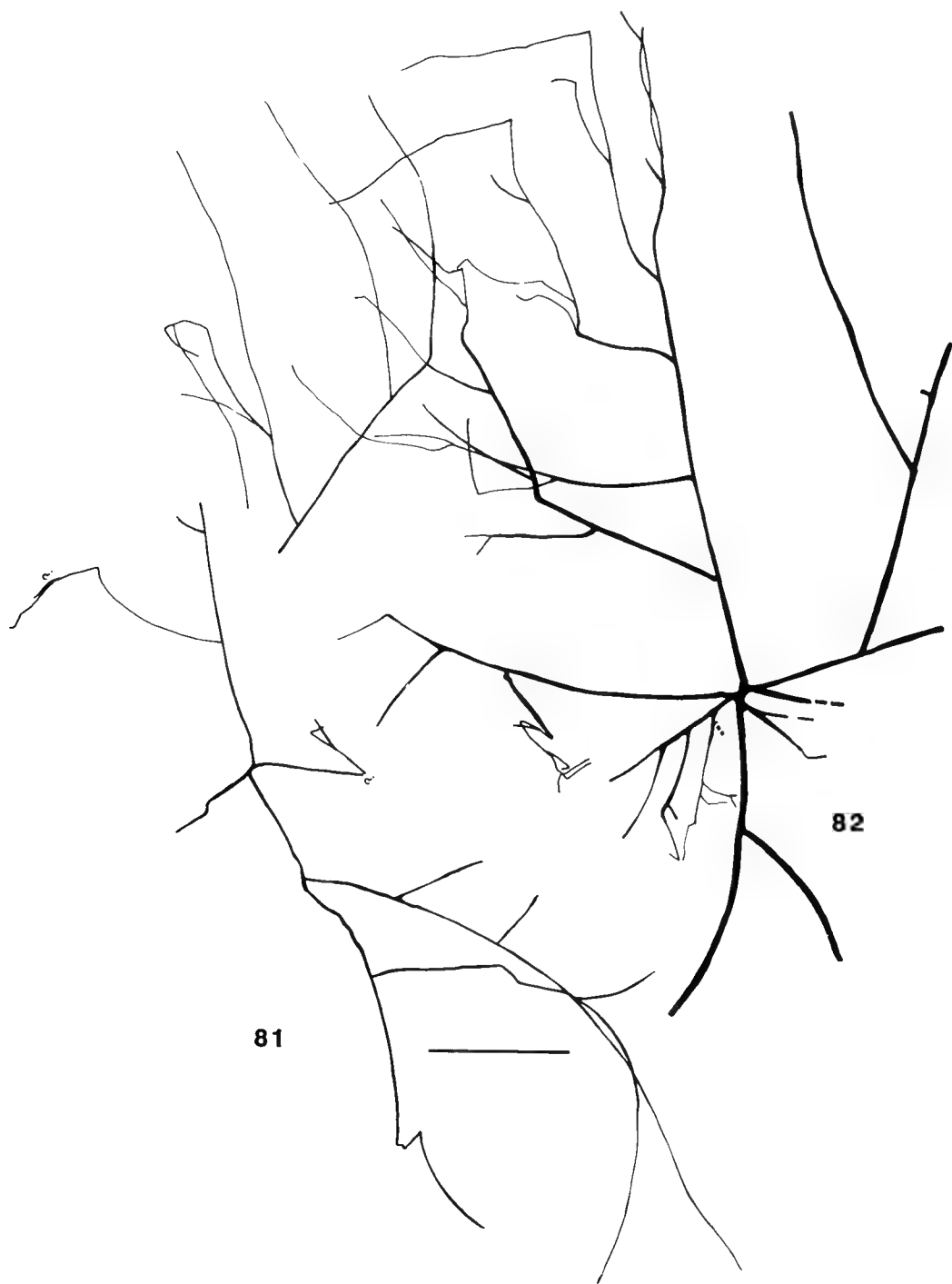
Figure 81. Trochograptus indignus Harris and Thomas, lectotype P83291.
