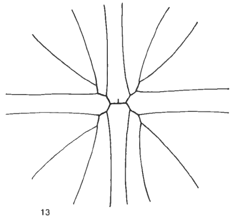
Figure 10. Goniograptus thureaui thureaui based upon P34847 (35817); 32 peripheral stipes; nodal formula 7/7/7/7.
