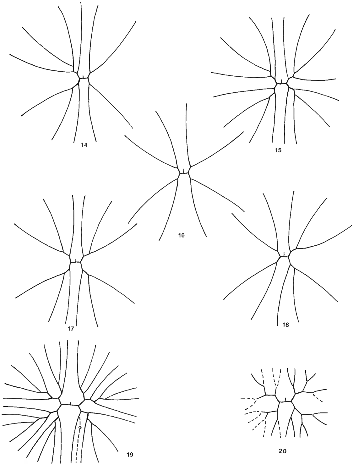
Figure 19. Praegoniograptus clonograptoides based upon the holotype P32169; 29 peripheral stipes; nodal formula 2/4; 4/0; 3/4; 3/2 ; seven monoproggressive dividing stipes. Bendigonian (Be1).
