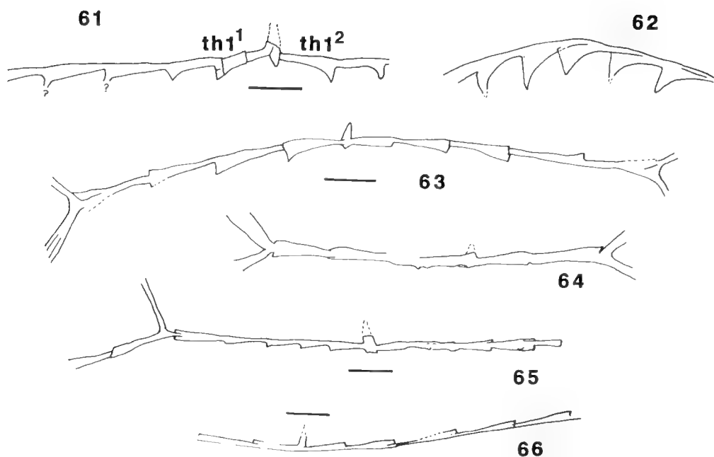
Figures 61, 62. Zygograptus irregularis Harris and Thomas, respectively proximal end of holotype, P32124, and distal thecae on 4th order stipe of same; 68 shows characteristic sigmagraptine proximal end. approx. Scalebar 1 mm.
