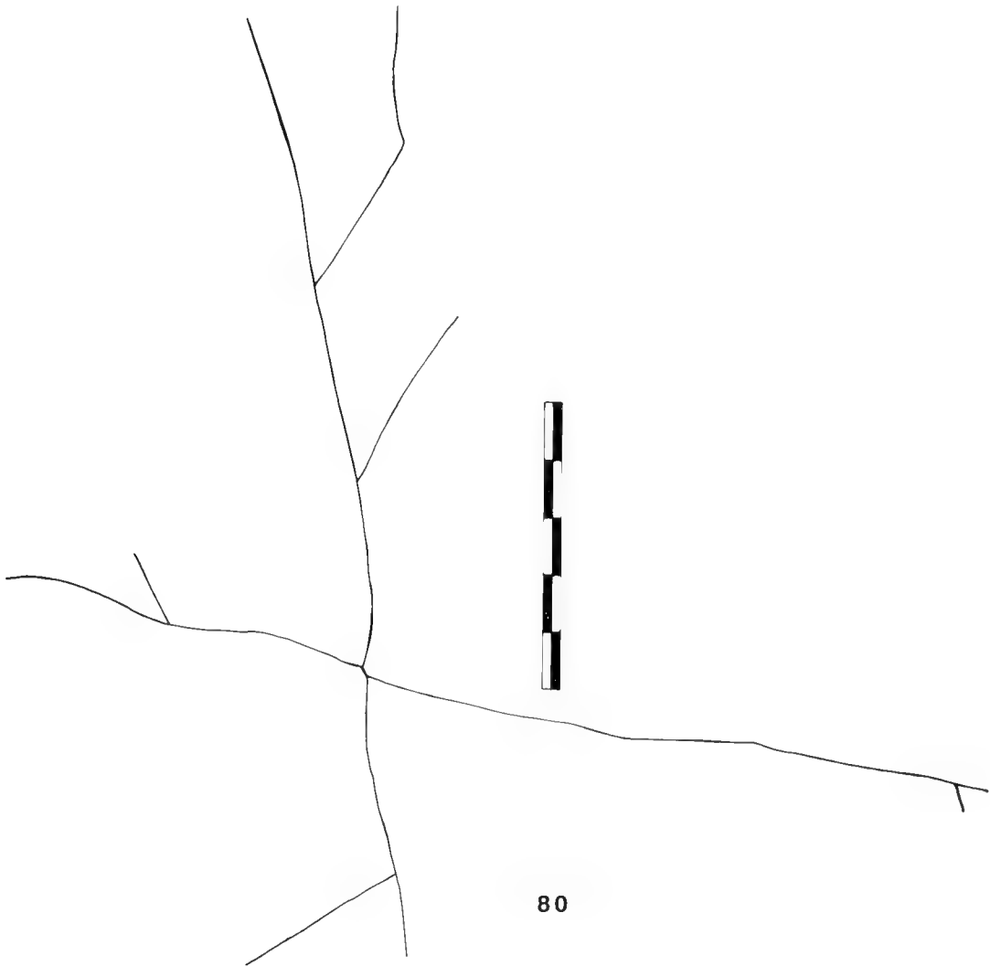
Figure 80. Trochograptus indignus Harris and Thomas, P83292, Scalebar 50 mm.
