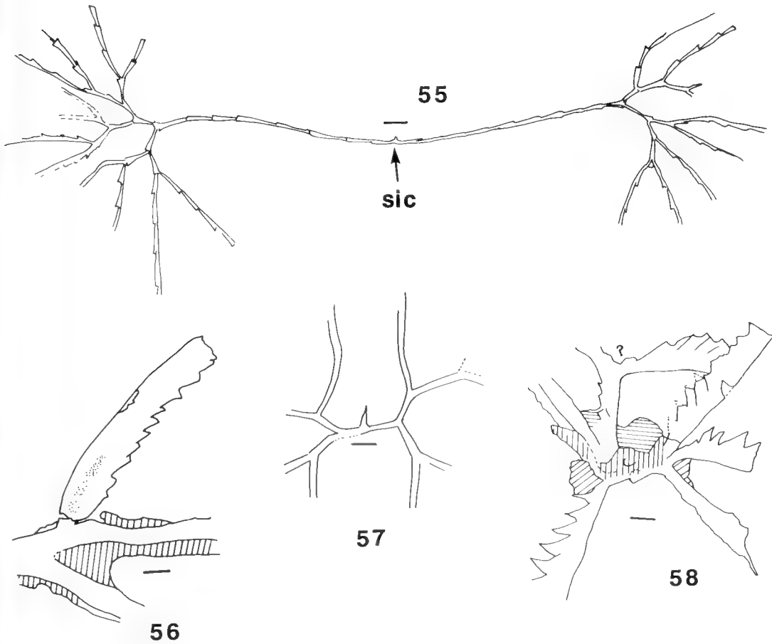
Figure 55. Zylograptus stewarti sp. nov., holotype, P73482. approx. Scalebar 1 mm.
