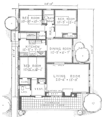
MODERN HOME No. 3306 ALREADY CUT AND FITTED
