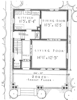
FIRST FLOOR 3315-B
