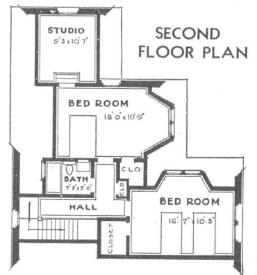
MODERN HOME No. 3308 ALREADY CUT AND FITTED
