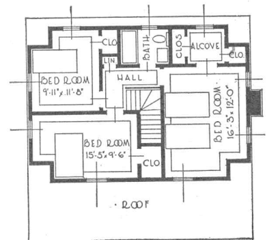
SECOND FLOOR PLAN If second bathroom is needed, it will work out nicely in alcove and closet space.
