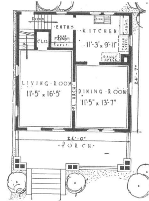
FIRST FLOOR 3315-A
