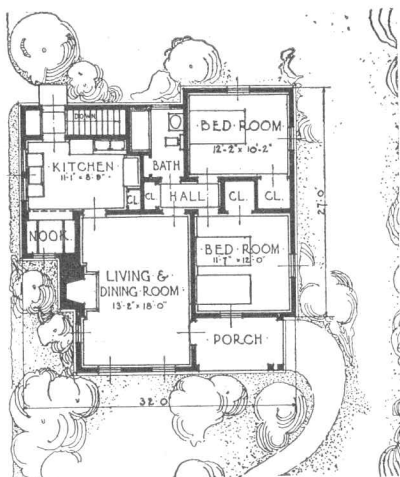
FLOOR PLAN
