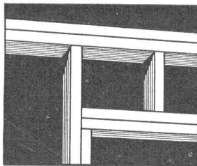
Double plates and double studs and headers around all window and door openings.
