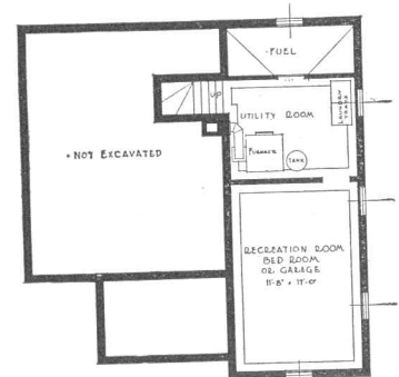
FOUNDATION PLAN
