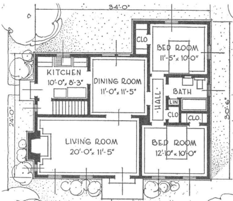
FLOOR PLAN No. 13354A
