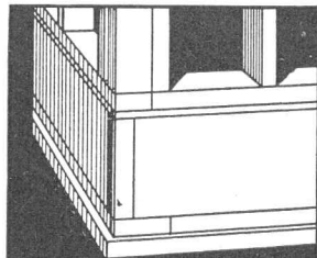
Three studs at all corners—studs on 16-inch centers.
