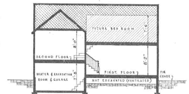
SECTION SHOWING FOUR FLOOR LEVELS
