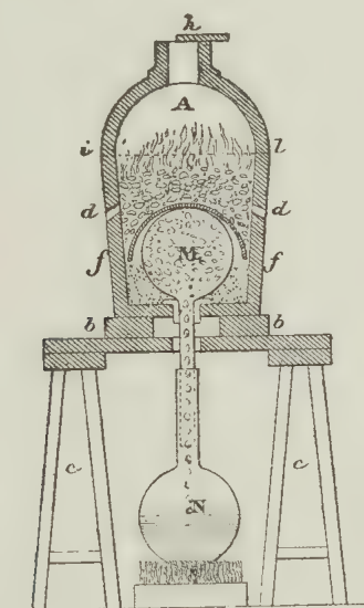
FIG. 69. Furnace with Payen's Receiver.
