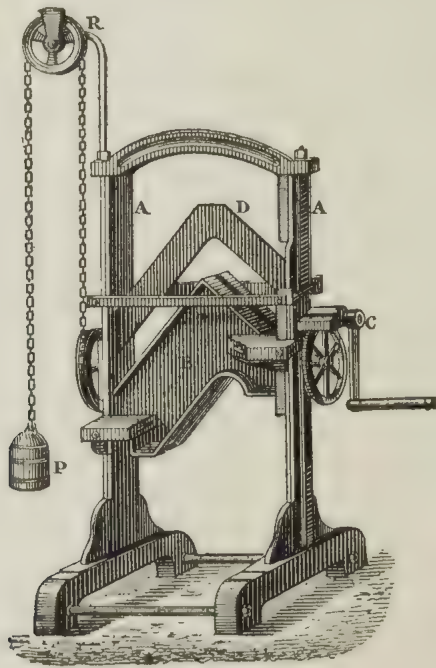
FIG. 119.—Bending Machine.
