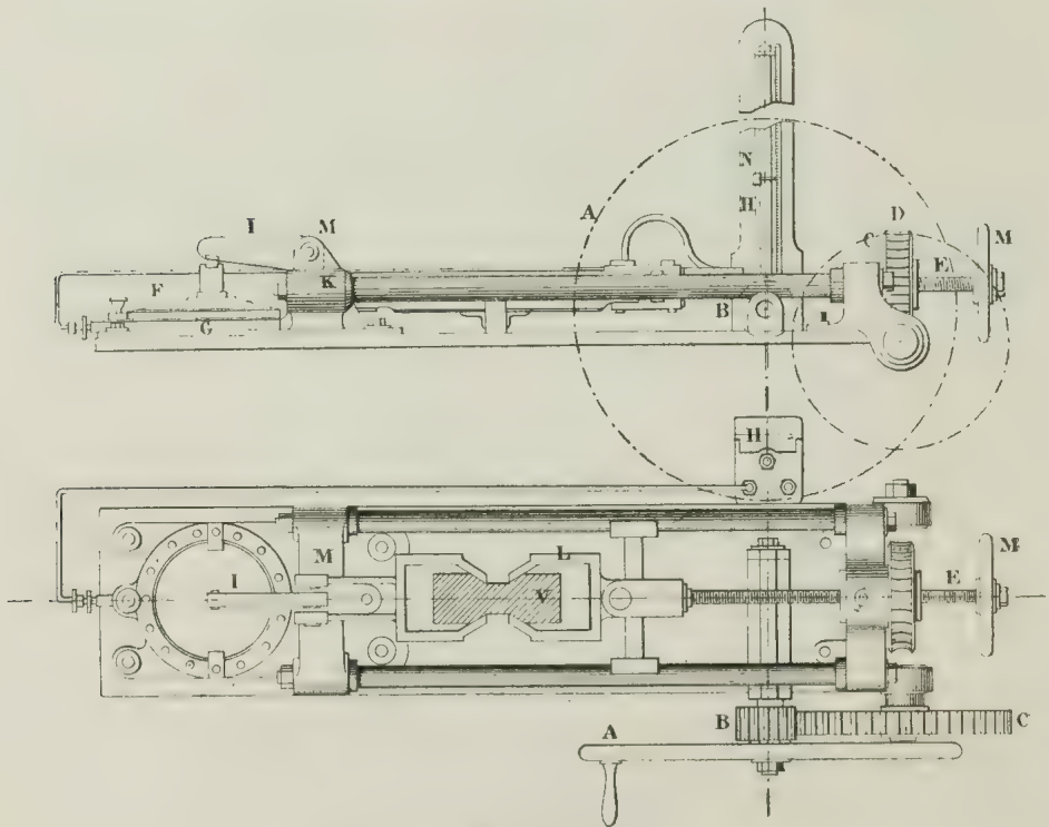
FIG. 93.—Thomasset Machine.
