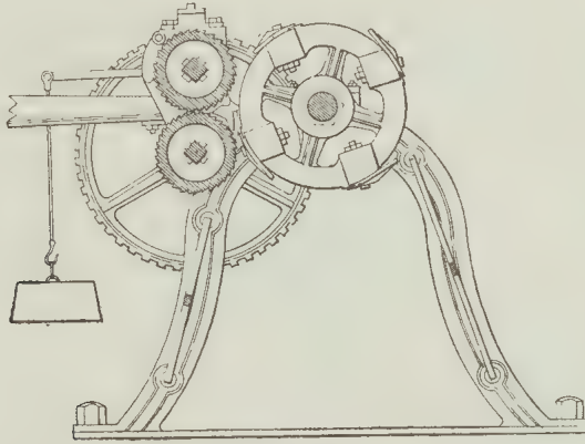
FIG 12.—Bark Cutter.
