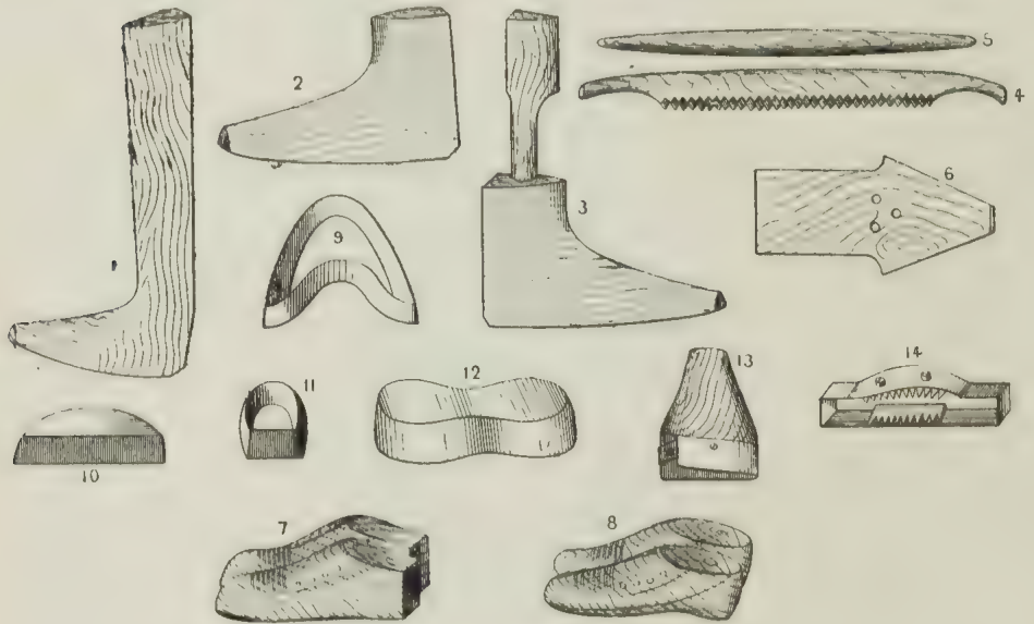
FIG. 120.—Shoemaker's Tools.
