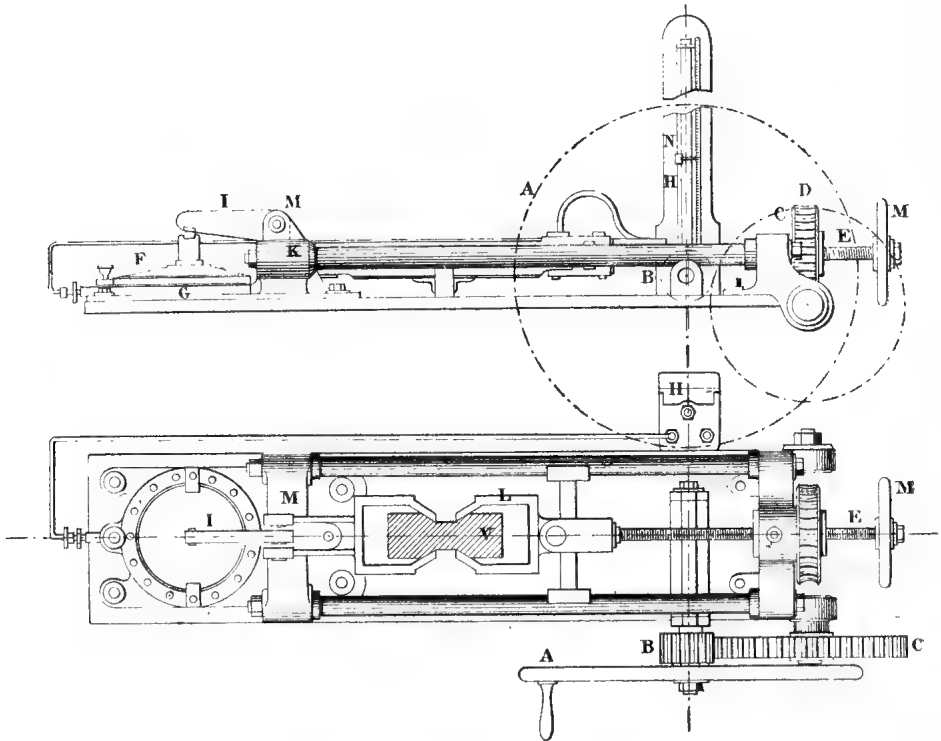
FIG. 93.—Thomasset Machine.
