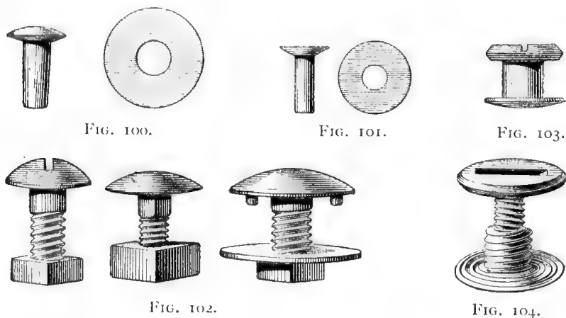
SOME RIVETS AND SCREWS USED IN BELT-MAKING.
