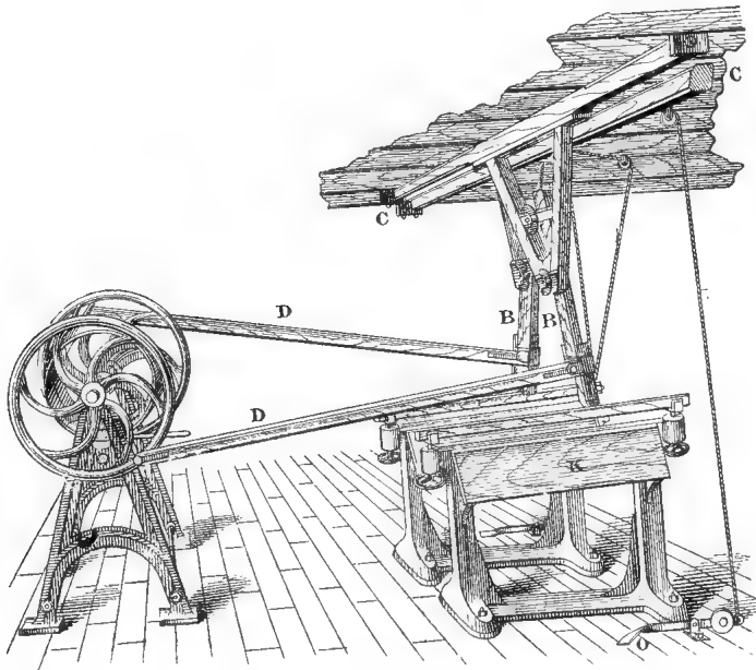
FIG. 84.—Glazing Machines.
