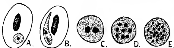
Fig. 131.— Proteosoma moruony (de Mollo & de Sá). A, young trophozoite; B, full-grown trophozoite; C, "Acton body," showing nuclear division; D, schizont; E, rosetta containing merozoites. (After de Mello and de Sá.)
