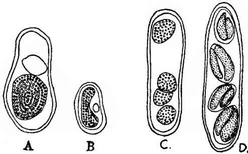
Fig. 96.— Eimeria southwelli Halawani. A , an immature pear-shaped oöcyst containing a large spherical zygote; B , an immature oöcyst retaining its hind-bulb to a slight degree; C , oöcyst containing four sporoblasts; D , fully mature oöcyst containing oval sporocysts. (After Halawani.)
