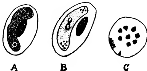
Fig. 116.— Hæmoproteus wenyoni de Mello, de Sá, de Sousa, Dias, & Noronha. A, female gametocyte ; B, male gametocyte ; C, extra-corpuseular schizont. (After de Mello and others.)
