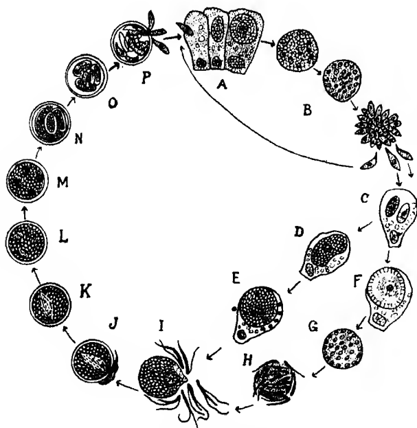
Fig. 80.—Life-cycle of Eimeria schubergi (Schaudinn). ( \times 400 .) A, entrance of a sporozoite in the gut epithelium of the host and growth of schizont; B, three stages in schizogony to form merozoites, which repeat schizogony; or C, become macro- and microgametocyte; D, E, formation of macro- gamete; F-H, formation of microgametes; I, in mature gametes and fertilization; J, secretion of a membrane round the zygote; K-N, stages in sporocyst formation; O, oöcyst containing four sporocysts, each with two sporozoites; P, escape of the sporozoites. (From Kudo, after Schaudinn.)
