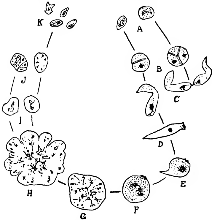
Fig. 151.— Babesia canis , development in the tick ( \times c. 1500). A, globular forms in the stomach of the tick; B, globular form showing split; C, club-shaped forms; D, "zygote," which passes through the stomach-wall; E-H, globular body in ovum or tissue-cells, which shows multiple fission; I, sporoblasts; J, formation of sporozoites; K, sporozoites in the salivary glands. (From Nuttall, after Christophers.)
