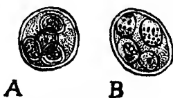
Fig. 87.— Eimeria knowlesi Bhatia. A, spherical oöcyst ; B, oval oöcyst. (After Knowles and Das-Gupta.)
