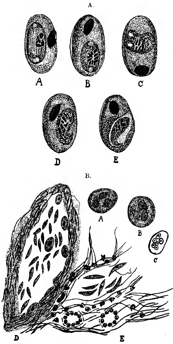
Fig. 65.— Haemogregarinus xavieri de Mello. A. In blood. A, B, oval forms; C, kidney-shaped form; D, elongate form with a short tail; E, elongate form within a capsule. B. A, cyst containing few schizonts; B, cyst containing six schizonts (merozoites); C, cyst containing six schizonts (merozoites); D, E, fusiform merozoites in the blood; A, B, C, in smears from lungs, spleen, and liver respectively; D, E, in section of a blood-vessel. (After de Mello.)
