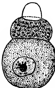
Fig. 30.— Stenophora ellipsoidea Chak. (After Chakravarti.)
