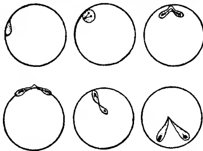
Fig. 148.— Babesia bovis (Babes). (After Nuttall.)
