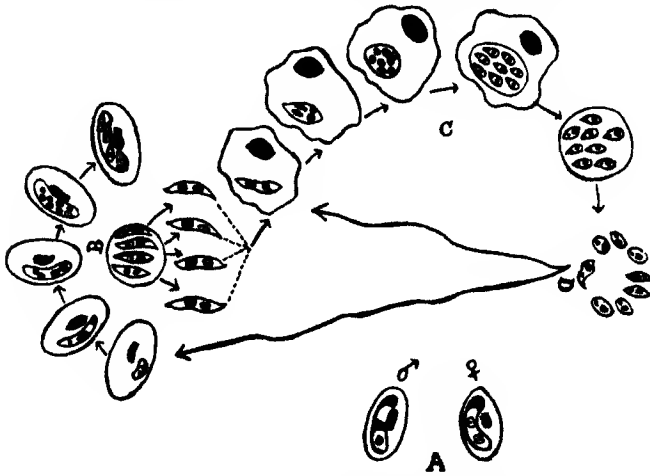
Fig. 71.—Life-cycle of Karyolysus jorgei de Mello & de Meyrelles. A , male and female gametocytes in peripheral blood; B , endoglobular cycle in capillaries producing macrocyysts with four merozoites; C , endothelial cycle in liver and lungs producing microcyysts with eight leishmaniform merozoites; D , free merozoites which may invade either the red cells or endothelial cells. (After de Mello and de Meyrelles.)
