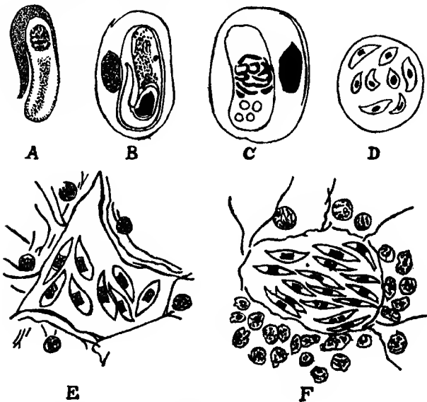
Fig. 52.— Hæmogregarina malabarica de Mello. A , free vermiform form; B , intra-corpuseular vermiform form; C , intra-corpuseular bean-shaped form; D , cyst, containing eight merozoites; E , F , larger merozoites found in the liver cell. A , B , C as seen in the blood; D , as seen in smears from the liver; E , F , as seen in sections of the liver. (After de Mollo.)
