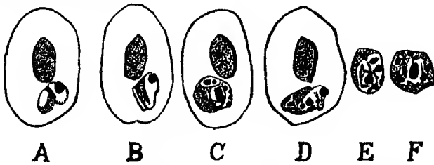
Fig. 130.— Proteosoma herodiadis (de Mello). A, ring-form; B, C, pyriform or rounded trophozoites; D, schizont; E, male gametocyte; F, female gametocyte. (After de Mello.)
