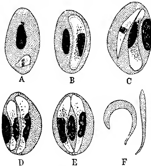
Fig. 61.— Hæmogregarina thomsoni Minchin. A , small intra-corporeal form; B , large intra-corporeal form showing the so-called "capsule"; C , a large and an intermediate-sized form in the same corpuscle; D , two large individuals lying side by side, both on one side of the nucleus; E , two large individuals embracing the nucleus between them; F , the free form. (After Minchin.)
