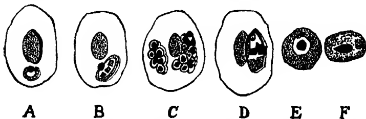
Fig. 128.— Proteosoma chloropsidis (de Mello). A, ring-form; B, full-grown trophozoite; C, rosettes; D, male gametocyte; E, F, female gametocytes. (After de Mello.)
