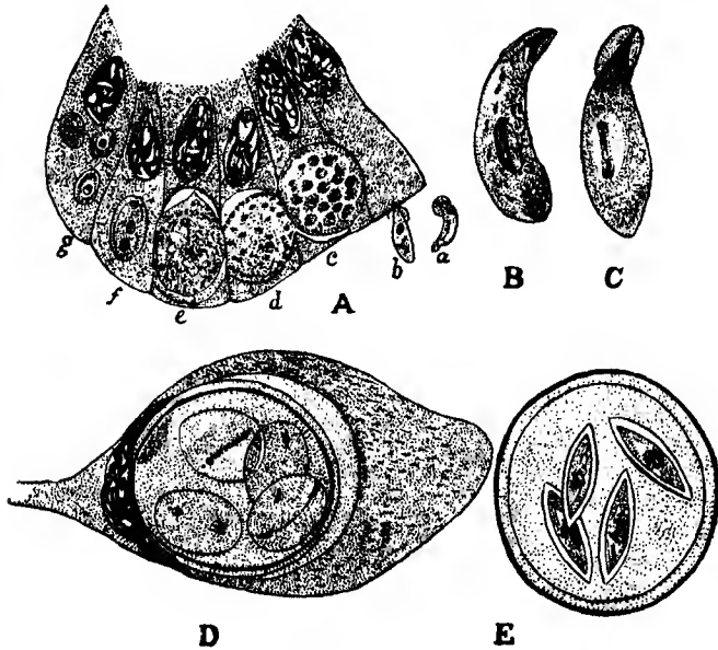
Fig. 88.— Eimeria laminata Ray. A, a portion of the transverse section of the small intestine (a, merozoite free in the lumen; b, merozoite entering a cell; c, macroschizogony; d, microgamete formation; e, macrogamete; f, microsizont; g, three merozoites in a cell); B, C, macro- and microschizonts showing laminae and a siderophilous area containing contractile elements; D, oocyst showing sporoblasts. E, mature oocyst. (After Ray.)
