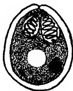
Fig. 168.—Spore of Myxobolus nodularis Southwell & Prashad. (After Southwell and Prashad.)
