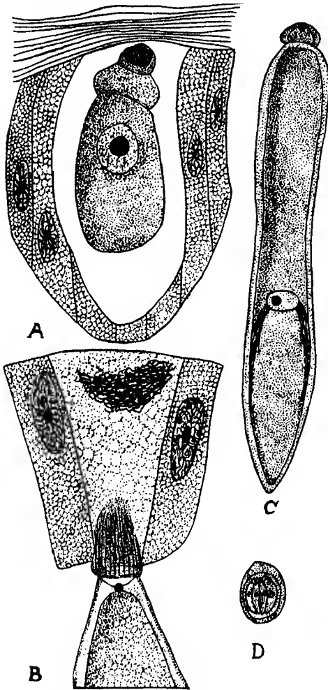
Fig. 32.- Hyalosporina cambolopsisae Chakravarti. A , young trophozoite growing intracellularly; B , older trophozoite, with epimerite attached by the collar and the tongue-like process thrust into the host-cell; protomerite is at the breaking-point, and shows the granule; C , adult trophozoite, with the nucleus tethered to the side-wall by the myonemes; D , mature sporocyst, showing the hyaline membrane, and eight sporozoites. (After Chakravarti.)
