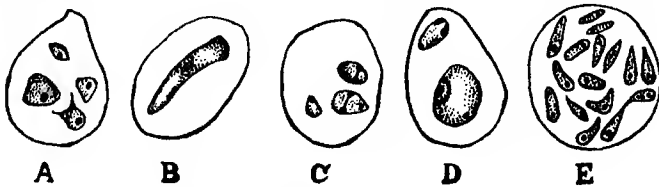
Fig. 154.— Babesia gibsoni (Patton). (From Wenyon, after Patton.)
