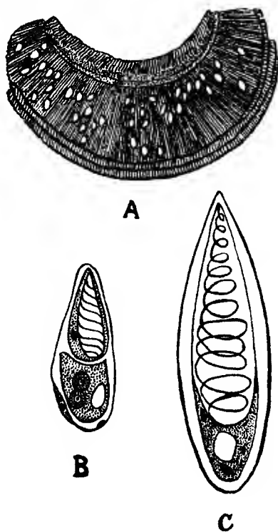
Fig. 169.— Thelohanellus rohitzæ (Southwell & Prashad). A , gill with cysts; B , young spore; C , mature spore. (After Southwell and Prashad.)
