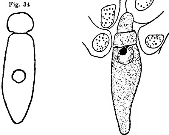
Fig. 34.— Leidyana gryllorum (Cuénot). (After Cuénot.)
