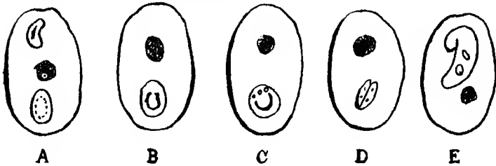
Fig. 49.— Haemogregarina laverani Simond. A, young amoeboid stage with a nucleus; B, young stage in which the cyanophil grains are dispersed in the form of a coil; C, young stage in which the cyanophil nuclear substance is in the form of a horseshoe; D, young vermicular stage; E, full-grown stage folded upon itself and showing two refringent granules. (From de Mello, after Simond.)
