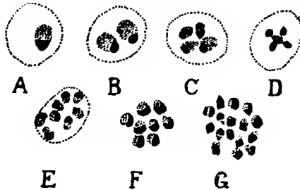
Fig. 146.— Theileria hirci Dsch. & Urod. A-E, intra-corpuseular forms; F-G, extra-corpuseular bodies showing multiple division. (After Sarwar.)
