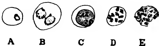
Fig. 138.— Plasmodium bubalis Shoather. A, young trophozoite; B, double infection with two trophozoites; C, large trophozoite; D, schizont; E, merozoites escaping from the corpuscle. (After Sheather.)
