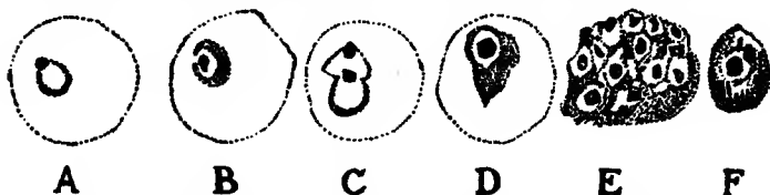
Fig. 141.— Plasmodium narayani de Mello & Dias. A, fimsy "ring"; B, compact "ring"; C, two "rings" in the same corpuscle; D, full-grown trophozoite; E, "rosette" showing schizogony; F, female gametocyte. (After de Mello and Dias.)
