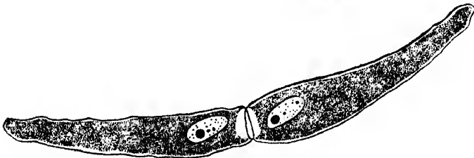
Fig. 19.— Extremocystis dendrostomi Setna. (After Setna.)
