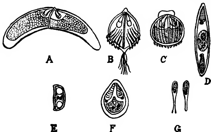
Fig. 164.—Some characteristic forms of spores of various MYXOSPORIDIA. A, Ceratomyxa truncata Thélohan; B, Chloromyxum leydigii Mingazzini; C, Sphaerospora rostrata Thélohan; D, Myxidium procerum Auerbach; E, Zschokkella acheilognathi Kudo; F, Myxobolus carassii Klokačewa; G, Hennequya gurleyi Kudo. ( \times 1500 .) (After Kudo.)
