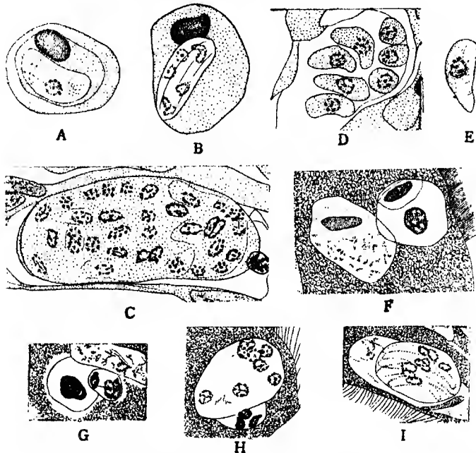
Fig. 56.— Hæmogregarina nicoria Castellani & Willey. A , bean-shaped Hæmogregarine , with circular type of nucleus; B , early stage of schizogony in the blood-stream; C , late stage of schizogony in the lung; D , fully-formed merozoites, only a very few of the total number formed shown in the section; E , free motile stage in the lumen of the intestine of the leech; F , microgametocyte lying closely applied to macrogametocyte; G , the microgametocyte giving rise to the microgamete nuclei, one of which fuses with the nucleus of the macrogamete; H , sporocyst with eight nuclei; I , sporocyst showing sporozoites. (After Robertson.)
