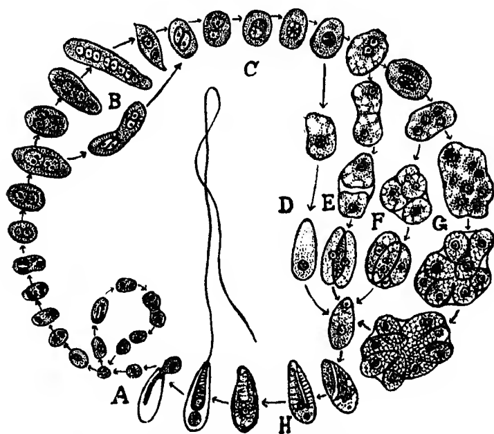
Fig. 171.—Diagram showing the probable development of a typical Microsporidian, Stempellia magna Kudo, \times 800 . A, amebula coming out from the spore in the mid-gut of Culicine larva; B, stages in schizogony or nuclear increase; C, sporont formation; D-G, formation of one, two, four or eight sporoblasts; H, transformation of a sporoblast into a nucleated spore with polar capsule. (After Kudo.)
