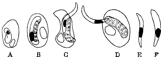
Fig. 54.— Hæmogregarina mirabilis Cast. & Will. A, intra-corpuseular form bent double; B, parasite within the capsule inside a corpuscle; C, D, parasite emerging from the cyst and the corpuscle; E, F, free forms. (After Castellani & Willey.)
