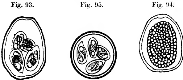
Fig. 93.— Eimeria smithi Yakimoff & Galouzo. (After Yakimoff and Galouzo.)
