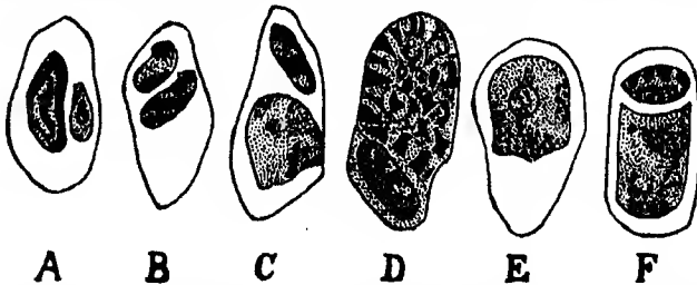
Fig. 132.— Proteosoma præcox (Grassi & Feletti). ( \times 2000 .) A , young ring-shaped trophozoite; B , C , larger trophozoites; D , schizont splitting into a number of merozoites; E , female gametocyte; F , male gametocyte. (After Wenyon.)
