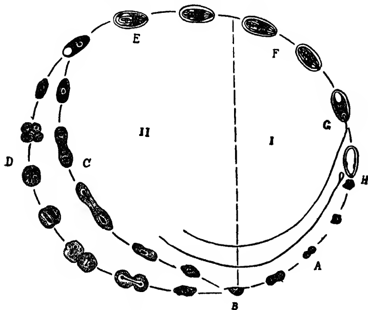
Fig. 174.—Life-cycle of Nosema bombycis Nägeli. I, extracellular stages; II, intracellular stages. A , planonts; B , meront; C , binary fission of meronts; D , multiple division of meronts; E , stages in spore formation; F , ripe spores in the midgut of a new host; G , extrusion of the polar filament; H , amœbula leaving the spore. (From Kudo, after Stempel.)
