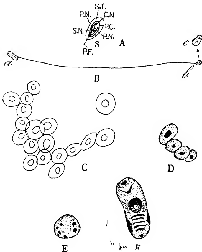
Fig. 175.—Stages in the life-cycle of Nosema etenocephali Kudo. A, fully developed sporocyst (C.N., capsulogenous nucleus; P.C., polar capsule; P.F., polar filament; P.N., parietal nucleus; S., spore; S.N., spore-nucleus; S.T., sporocyst); B, germination with extruded filament, with a planont at its extremity (a, sporocyst; b, planont; c, same, highly magnified); C, colony of planonts; D, division of meronts to form a chain-like group; E, division of meronts to form a cluster; F, capsule and polar filament (After Korke.)
