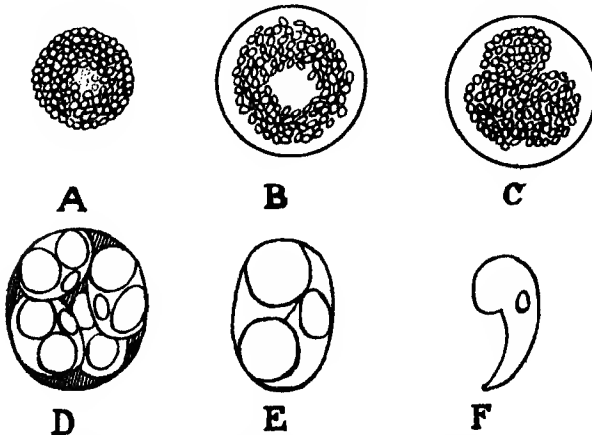
Fig. 89.— Eimeria legeri (Simond). A , growing macrogamete; B , encysted condition; C , oöcyst containing sporoblasts; D , oöcyst containing sporocysts; E , fully developed sporocyst; F , sporozoite. (After Simond.)
