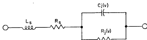
Fig. 62. Tunnel-diode equivalent circuit for microwave frequencies.
