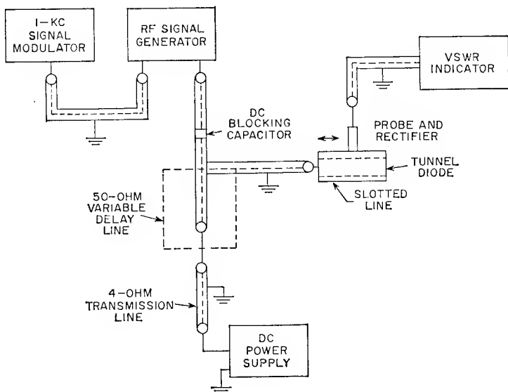
Fig. 133. Test setup for measuring inductance.
