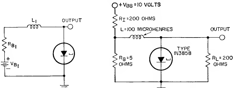
Fig. 29. (a) Basic tunnel-diode astable multivibrator and (b) practical circuit.
