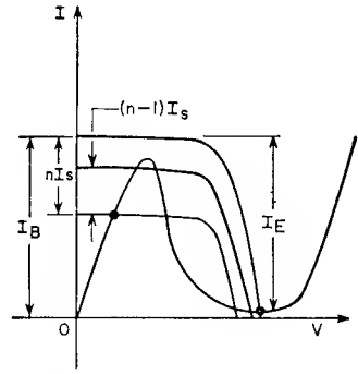
Fig. 59. AND-gate biasing.
