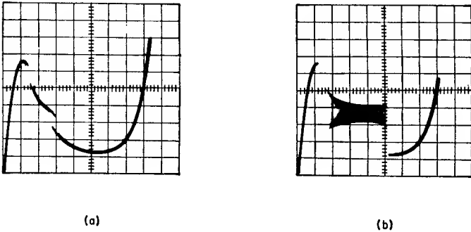
Fig. 117. Presence of imperfections in diode characteristic.
