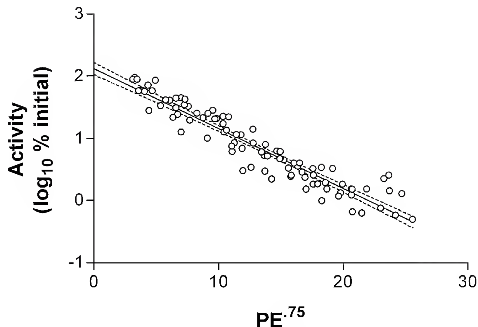
FIGURE 2.11 Linear model relating pasteurization effect (PE) and residual activity of lactoperoxidase during high-temperature short-time (HTST) pasteurization of bovine milk.
