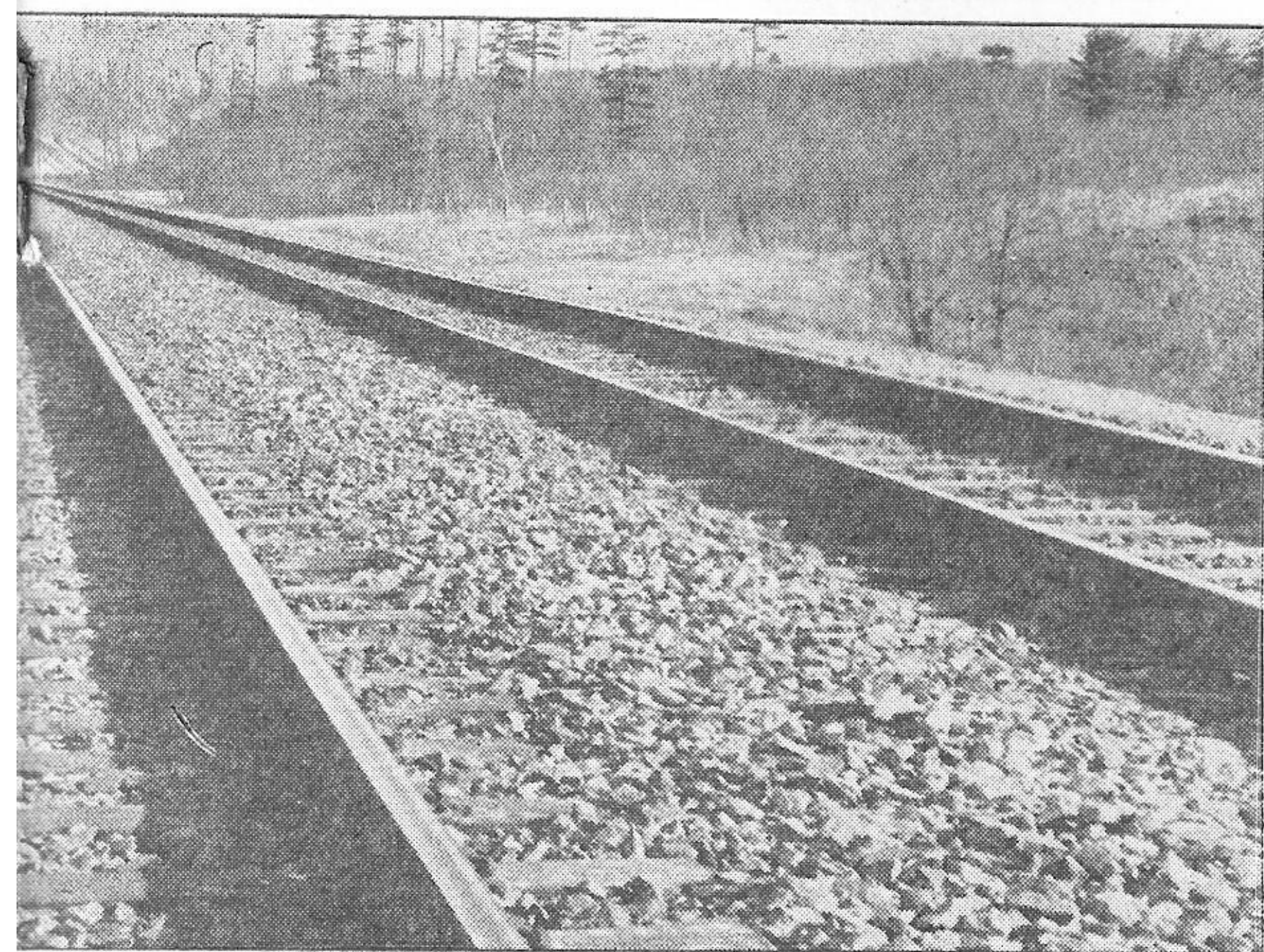
Secured to Creosoted Ties by M. & L. Fastenings
