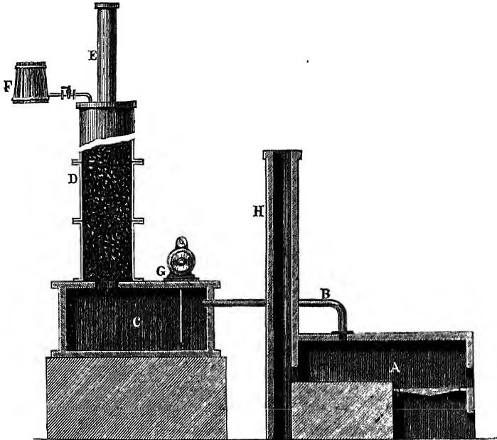
FIG. 6.—A, Sulphur burner; B, stove exit pipe; C, collecting tank; D, coke tower, consisting of twelve earthenware pipes, each 760 mm. (30 in.) long; E, draught regulator; F, water tank; G, steam pump for acid; H, chimney to sulphur burner.
