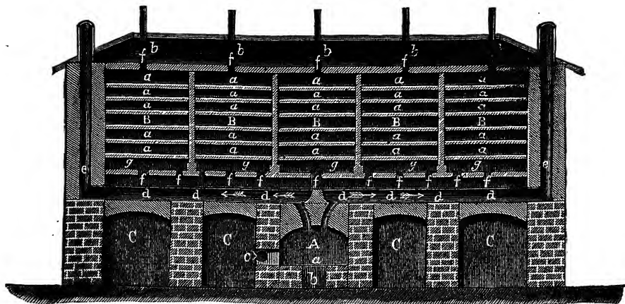
FIG. 1.—Vertical section of the furnace, with drying-stoves for heated air. A , Furnace; a , hearth; b , ashpit; c , door; d , flues; e , chimney; f , air passages; g , covering plates. B , Drying-stoves; a , shelves; b , pipes for the moist air. C , Workrooms.
