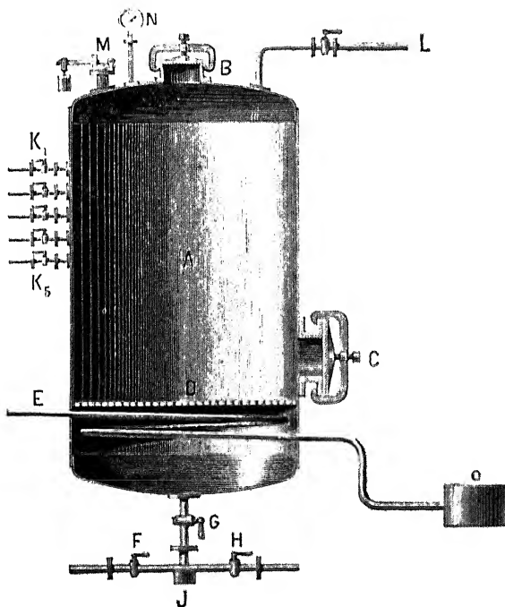
FIG. 7.— A , iron pan, lined with lead in order that the bleaching process may be conducted in it; B , feed opening; C , outlet; D , perforated bottom; E , steam coil connected with the steam trap c ; F , steam pipe; G , drain cock, shut during boiling; H , cock on drain pipe; J , water outlet; K 1 - K 5 , run-off cocks for fat and oil; L , pipe conveying the noxious gases to the boiler fire; M , safety valve; N , pressure gauge.
