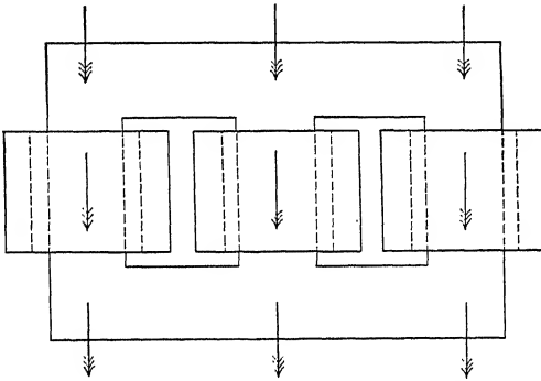
FIG. 208.—Core-type transformer.
