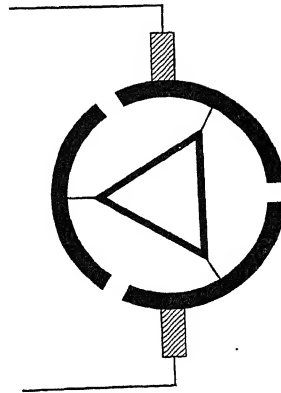
FIG. 107.—Three-phase delta-connected rectifier.
