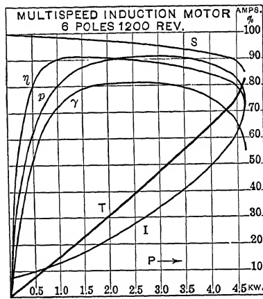
FIG. 10.—Load curve of multi-speed induction motor, middle speed, six poles.
