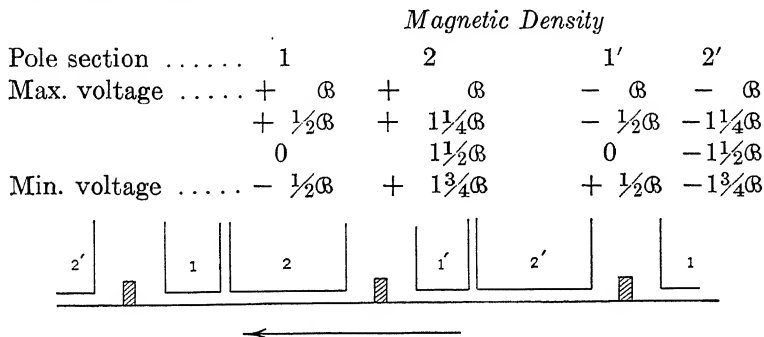
FIG. 211.—Two-section pole for variable-ratio converter.
