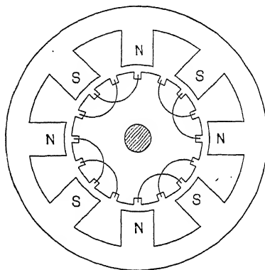
FIG. 134.—Revolving armature alternator
