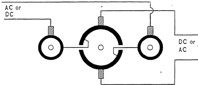
FIG. 73.—Rectifying commutator.
