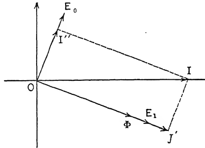
FIG. 177.—Single-phase commutator-motor improvement of power-factor by introduction of lagging e.m.f. of rotation.
