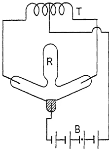
FIG. 101.—Mercury-arc rectifier, contact making.
