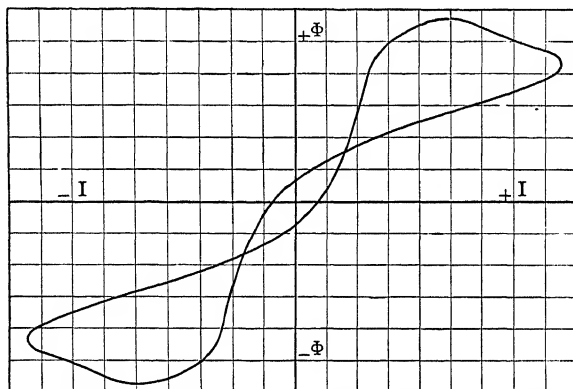
FIG. 131.—Hysteresis loop of reaction machine as generator.
