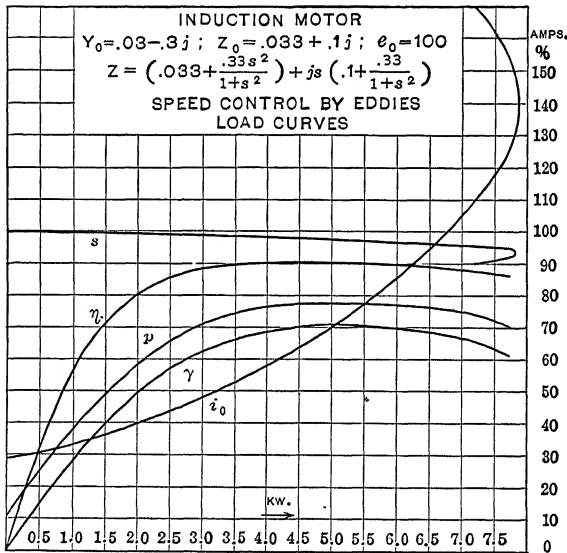
FIG. 5.—Load curves of induction motor with eddy-current starting device.
