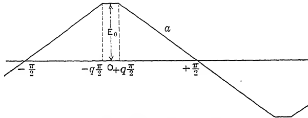
Fig. 209.—Y c.m.f. wave.
