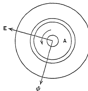
FIG. 125.—Diagram of machine with uniform reluctance.
