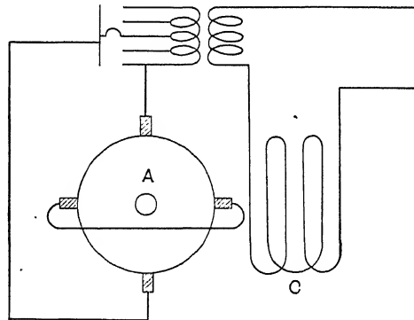
FIG. 184.—Winter-Eichberg motor.
