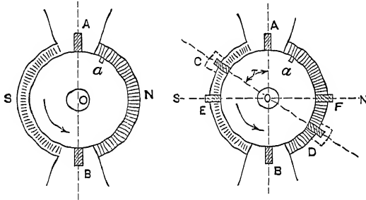
FIG. 195.—Diagram of commutating machine with brushes in the magnetic neutral.
