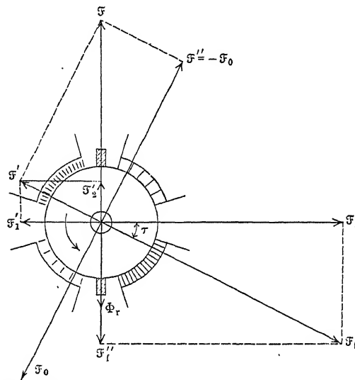
FIG. 203.—Diagram of m.m.f.s. in split-pole converter.
