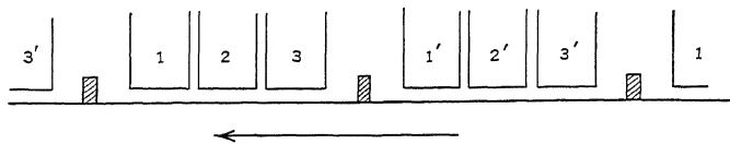
Fig. 210.—Three-section pole for variable-ratio converter.
