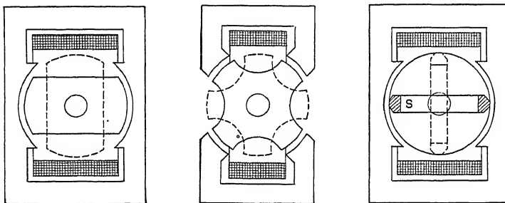
FIG. 128.—Synchronous-induction motor as reaction machine.
