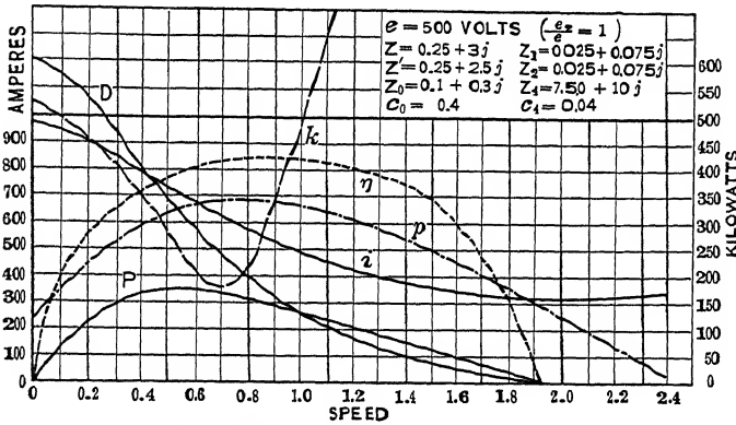
Fig. 192.—Repulsion motor, secondary excitation.
