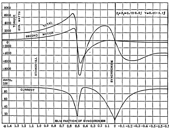
Fig. 18.—Speed torque curves of concatenated couple with low resistance secondary.
