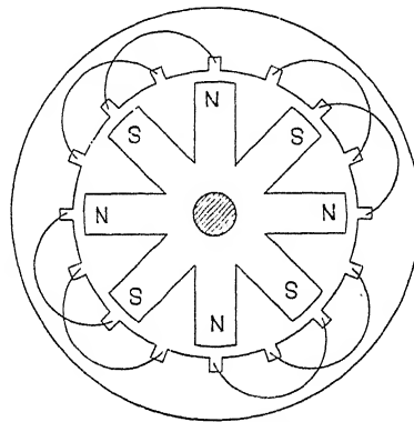
FIG. 135.—Revolving field alternator.
