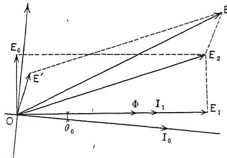
FIG. 179.—Single-phase commutator-motor diagram with secondary excitation.
