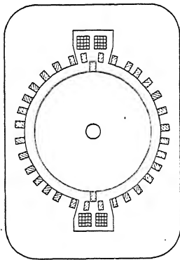
FIG. 159.—Completely distributed compensating winding.
