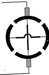
FIG. 109.—Quarter-phase rectifier with independent phases.
