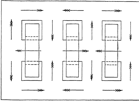
FIG. 207.—Shell-type transformers.
