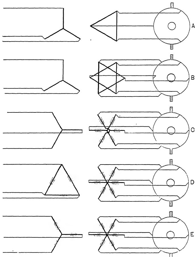
FIG. 206.—Transformer connections for varying the e.m.f. ratio by superposition of the third harmonic.
