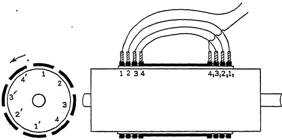
FIG. 224.—Multi-conductor unipolar machine, cross-section.
