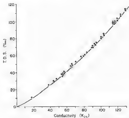
Fig. 2. Relationship between conductivity ( K_{25} ) and TDS (%w/w). The line represents the regression equation of Williams (1966). The points are values of K_{25} and TDS by weight for samples from the Coorong lagoons.
