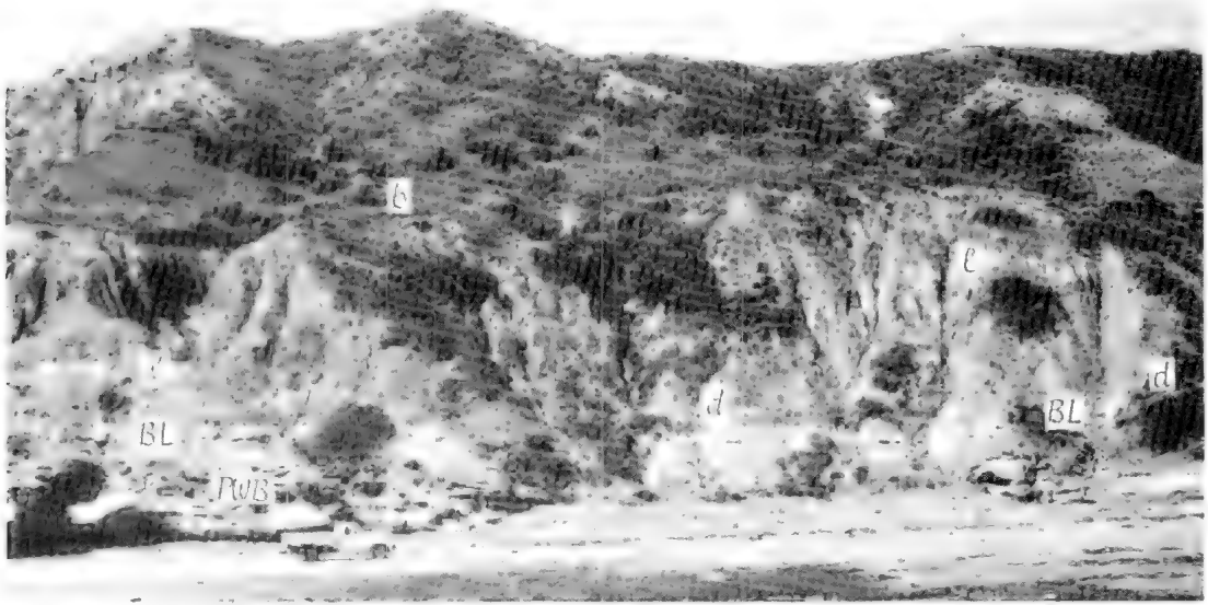
Fig. 4. View of sediments involved in older slump which occurred through a depression in the Port Willunga Formation (PWB). Upthrusting of Burnham Limestone (BL), dolomite layer (d) and other light-coloured sediments (l) is especially notable on right side of photograph. Minor bench level about half way up cliff at (b) represents remnant of a once more extensive slump surface.
