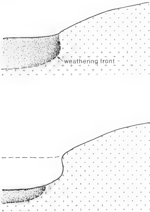
Fig. 10. Development of flared slopes.
