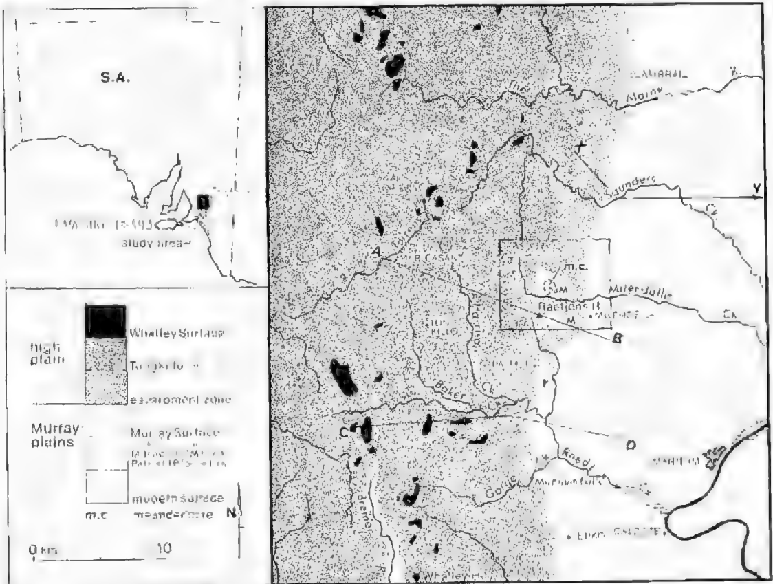
Fig. 1. Physiographic regions of part of the eastern Mount Lofty Ranges, and (inset) location map. The area around Ruetjens Hill and depicted in Fig. 5b is indicated. A-B and C-D are the lines of section shown in Fig. 5a, and X-Y the section represented in Fig. 7.
