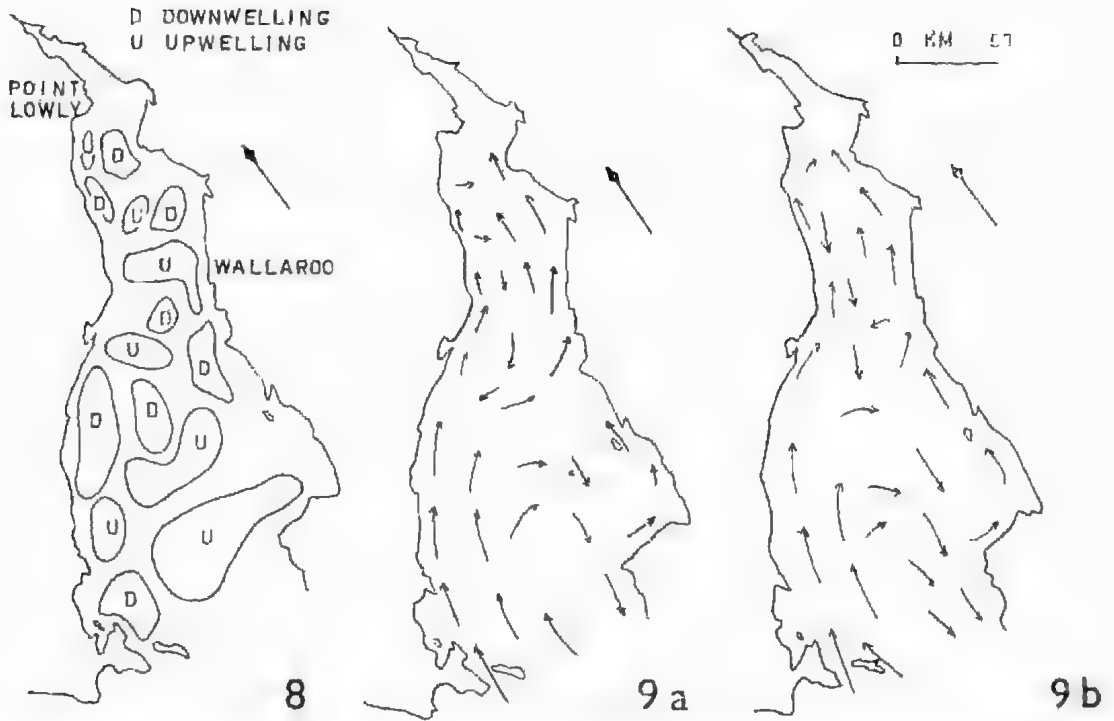
Fig. 8. Predicted regions of up- and down-welling due to thermohaline currents in Spencer Gulf. Fig. 9. Predicted currents in the presence of a 14 ms -1 SW wind. (a) Surface, (b) Bottom.
