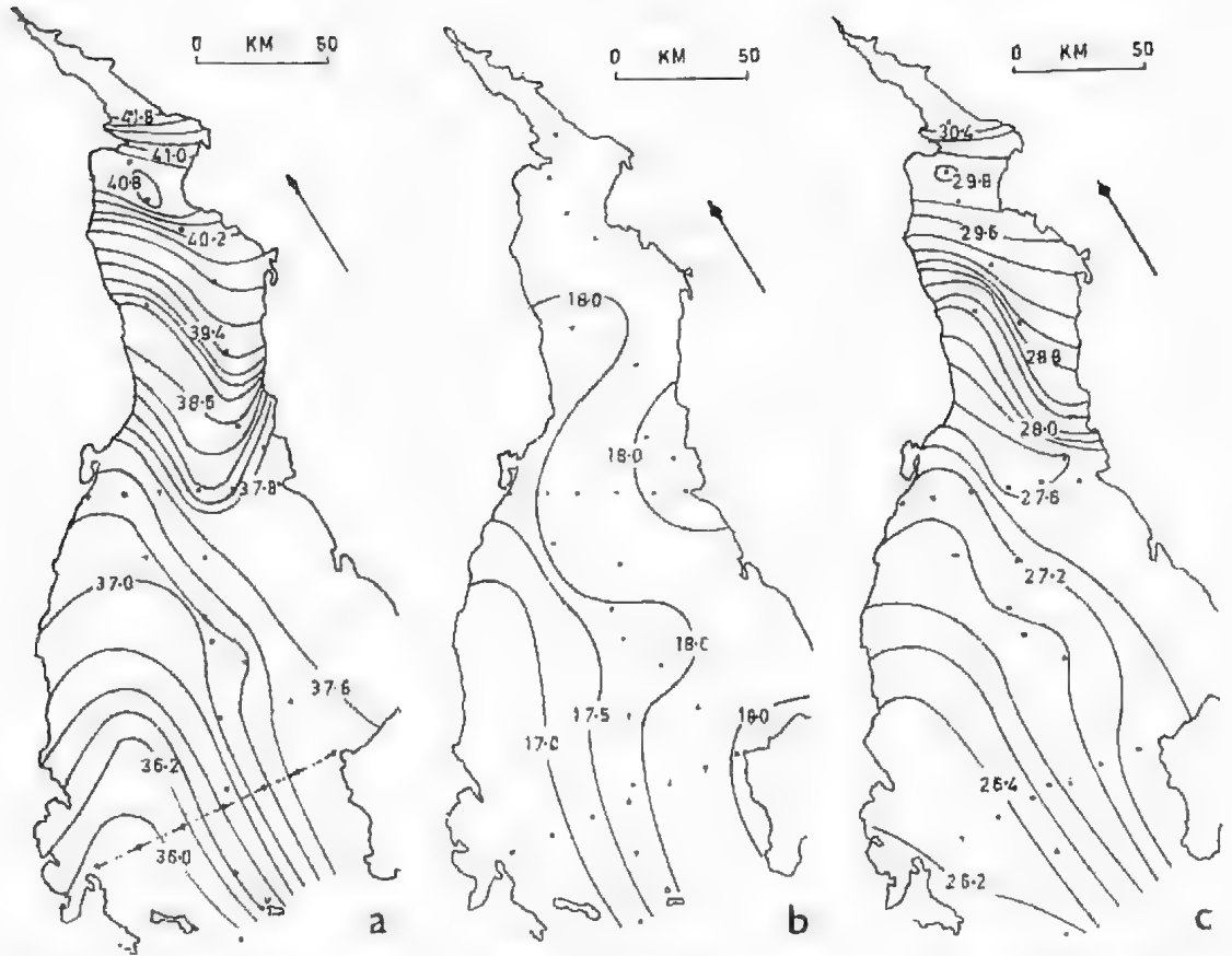
Fig. 3. Horizontal depth-average distributions in Spencer Gulf. Data taken from CSIRO Aust. 1968c. (a) Salinity (‰), (b) Temperature ( ^{\circ}\text{C} ), (c) \sigma_t .
