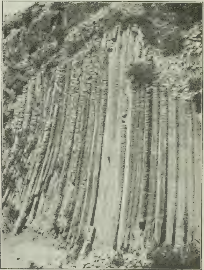
26. — "The Organ Pipes," Jackson's Creek, near Sydney, N.S.W. The illustration on facing has contained the term columns. These are 10 ft. high. (Phot. by Mr. H. J. Gray.)
