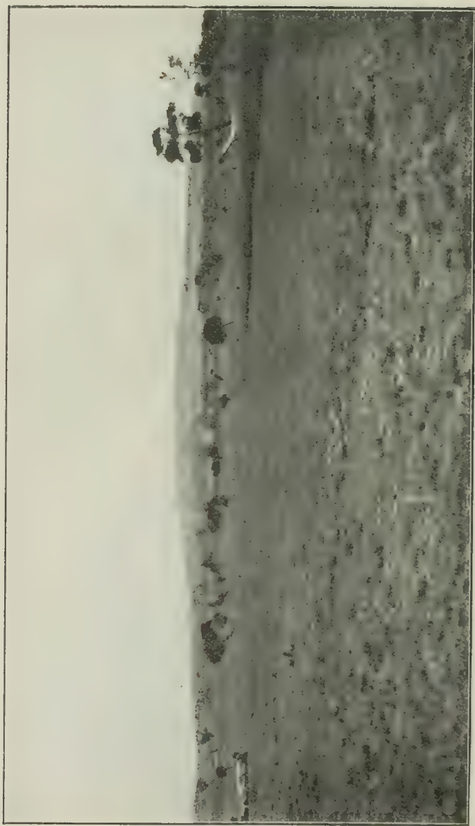
34.—Near Gnarwarrie, showing vegetation of red sands—gums, sheoaks, sword-grass. Mt. Moriac (volcanic) in the background.
