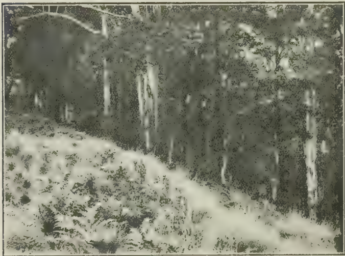
39. The forest on the southern slope of Mount Buninyong. The porous cinder heap holds water well.
