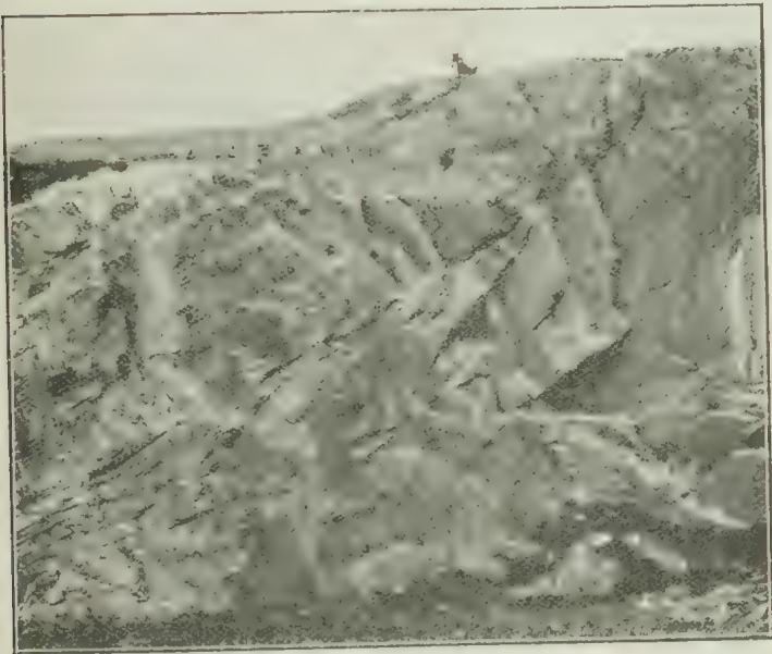
15. Auburn Brick Pit, showing the tilted bed-rock. The layers were originally horizontal.
