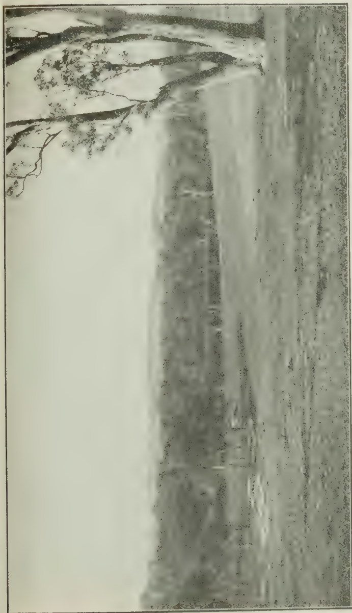
12. The Yarra valley above Alphington. Notice the wide valley as compared with that shown in fig. 11.
