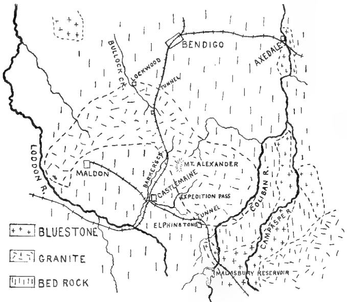
28.—Map of the country bordering the railway line from Malmsbury to Bendigo. The crescent-shaped area of granite is surrounded by a wall of hardened rock through which tunnels were necessary.
