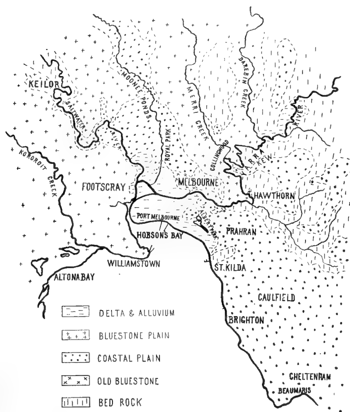
7.—Geological map of the Melbourne district.
