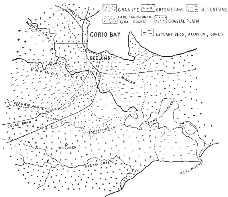
31.—Geological map of the Geelong district.
