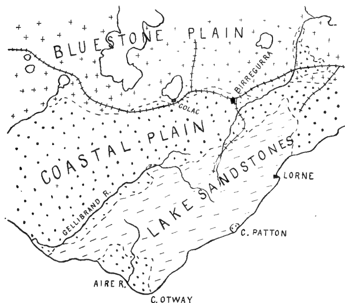
25.—Map of the Otway district and the country to the north. The lake sandstones, which formed the Otway Ranges (now 2,000 ft. high) stood up as an island in the sea in which the rocks of the coastal plain were laid down. The bluestone to the north covers a large area of these marine coastal plain beds.
