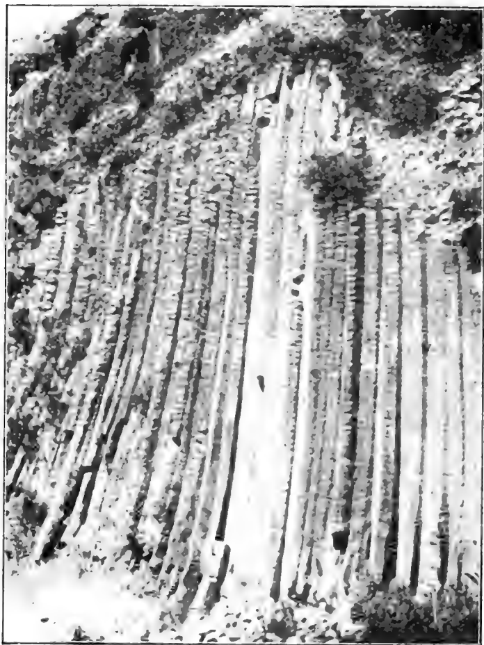
26107 The Queen's Pipe, Jackson's Creek, near S. C. Hill. The 90° dip is cutting, but common to the whole locality. These are 60 ft. in dip. (Phot. by Mr. H. J. Caspary.)
