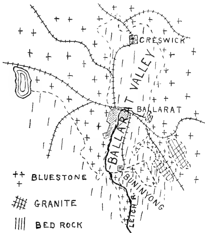
38.—Map showing the Ballarat Valley.
