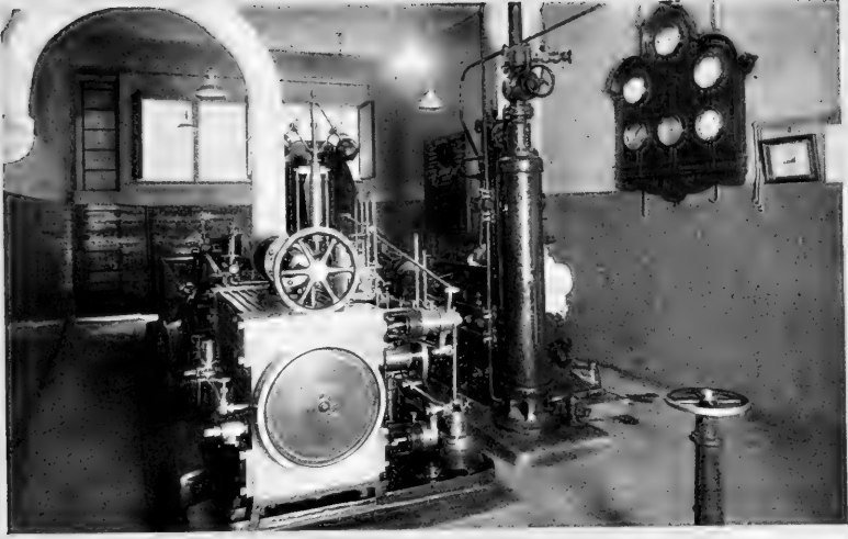
REFRIGERATING PLANT OF THE SUPPLY DEPARTMENT.
