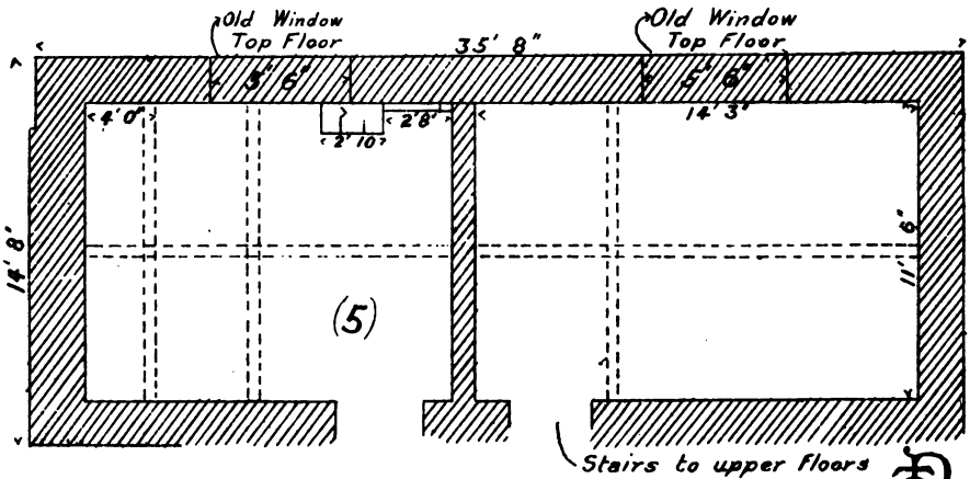
PLAN OF OLD BUILDING
