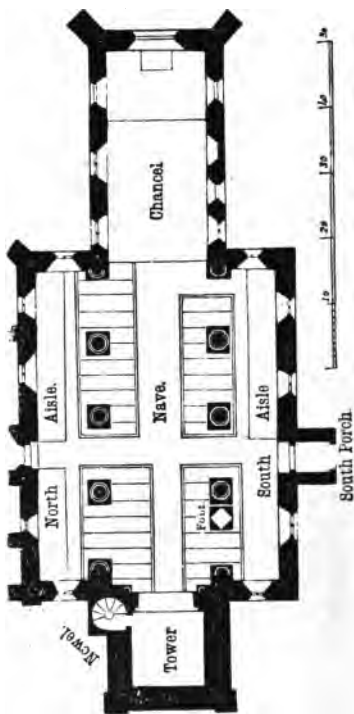
Plan, Garsington, Oxon.
