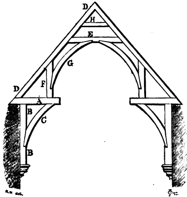
Hammer-beam Roof.
