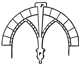
Section of a roof showing a Pendant.
