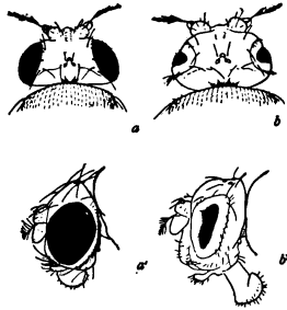
FIG. 31. Mutant race of fruit fly called bar to the right (normal to the left). The eye is a narrow vertical bar, the outline of the original eye is indicated.
