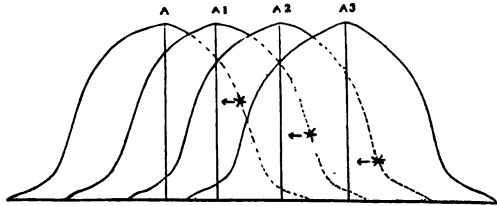
FIG. 79. Curves showing how (hypothetically) selection might be supposed to bring about progress in direction of selection. (After Goldschmidt.)
