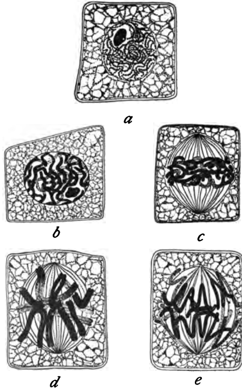
FIG. 46. A series of cells in process of cell division. The chromosomes are the black threads and rods. (After Dahlgren.)
