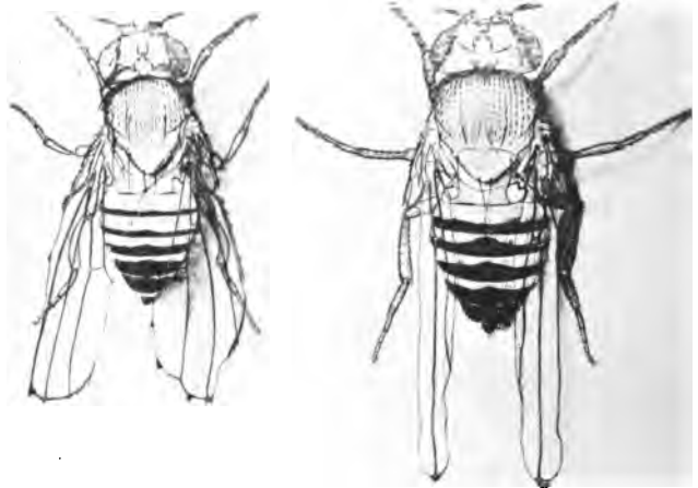
FIG. 84. Two flies showing beaded wings.
