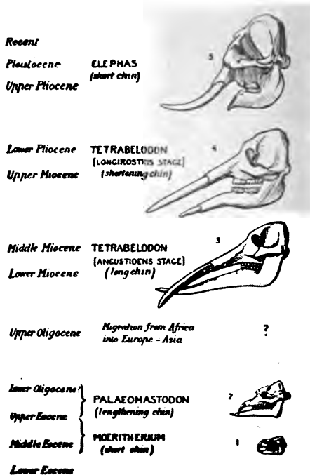
FIG. 93. Evolution of elephant's skulls. (After Dendy.)
