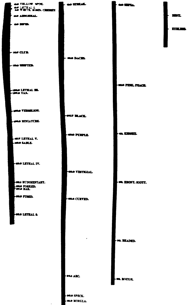
FIG. 67. Map of four chromosomes of D. ampelophila locating those factors in each group that have been most fully studied.
