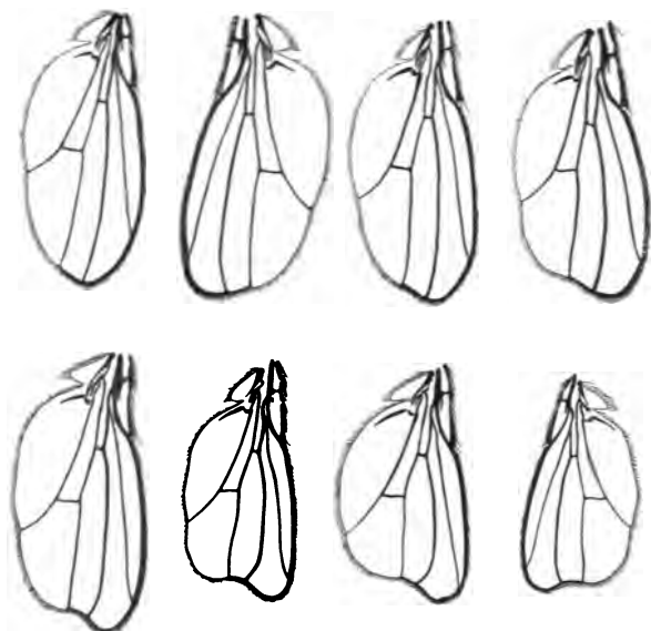
FIG. 83 b. Series of wings of different length shown by truncate stock of D. ampelophila .
