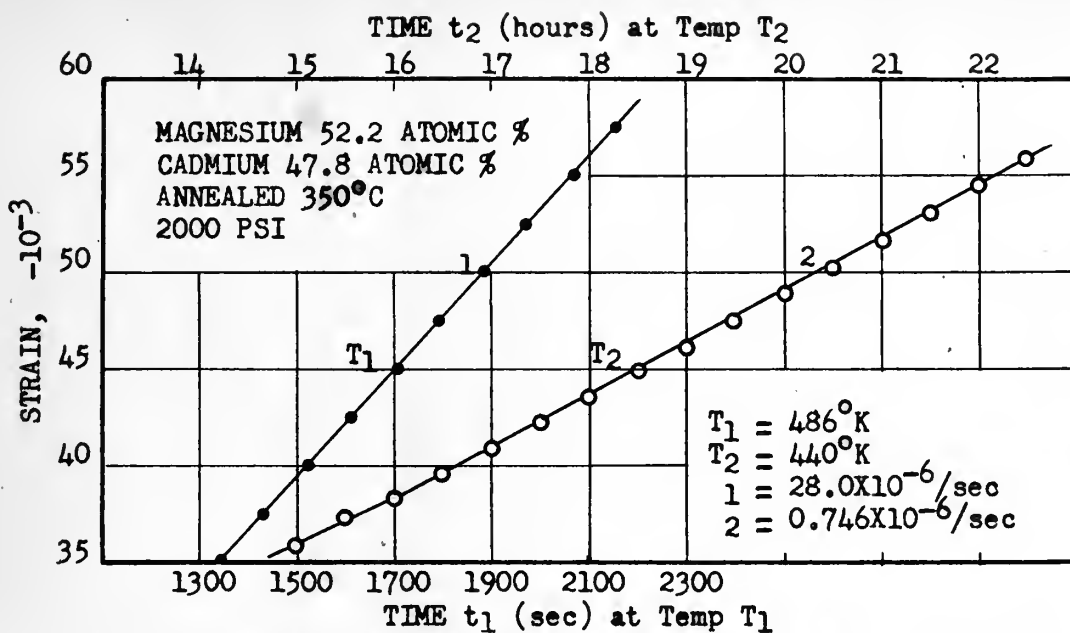
FIG. 12 STRAIN vs TIME FOR 52.2 ATOMIC % Mg and 47.8 ATOMIC % Cd. ANNEALED 350°C
