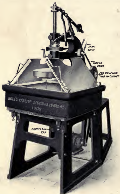
Fig. 111. The Holt Etching Machine.
