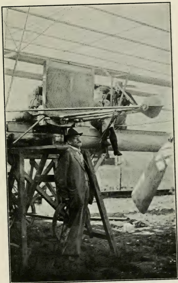
PART OF CAR AND ONE OF THE MOTORS — 1909.
