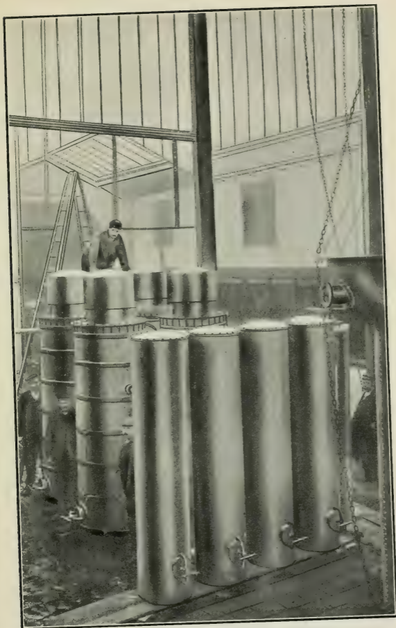
ASSEMBLING THE PARTS OF THE GAS APPARATUS, PARIS — 1910.
