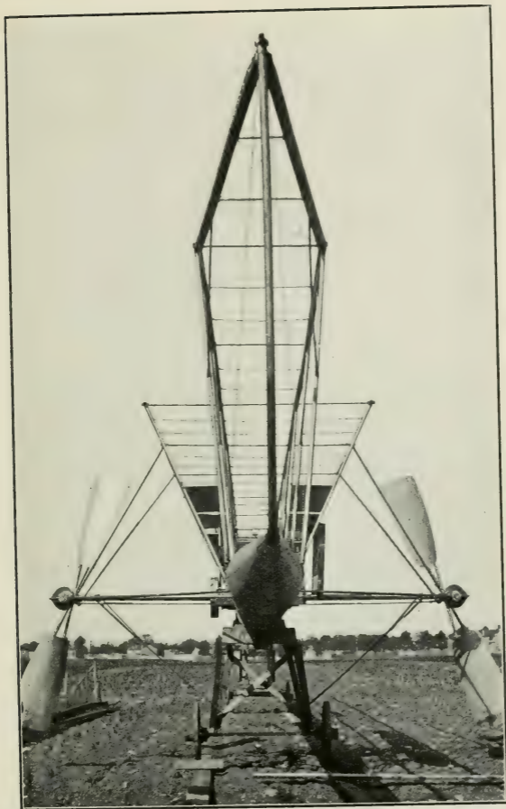
THE STEEL CAR OF THE AIRSHIP AMERICA — 1907.
