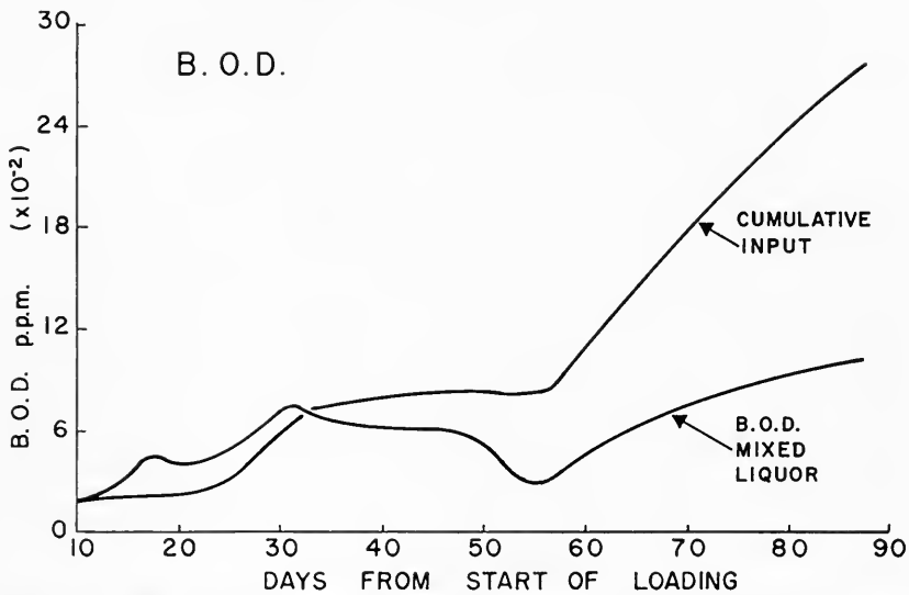
BOD 5 of the lagoon mixed liquor and cumulative (BOD 5 input minus BOD 5 irrigated). (Fig. 25)
