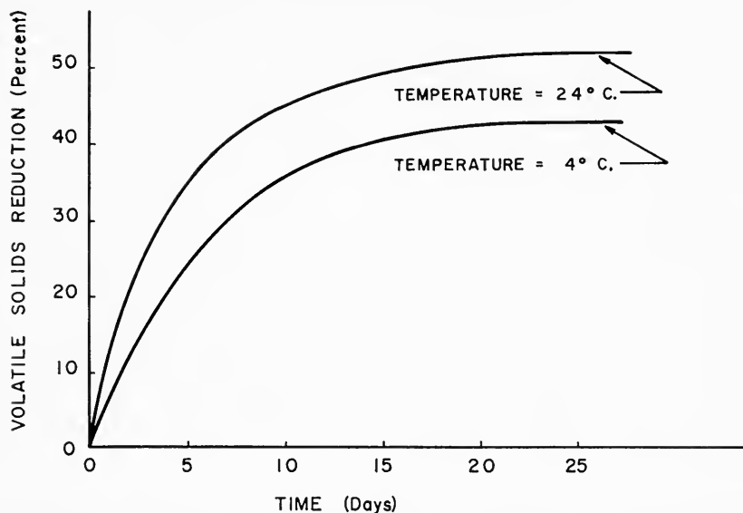
Comparison of the effect of two temperatures ( 4^{\circ} C. and 24^{\circ} C.) on volatile solids reduction. (Fig. 8)
