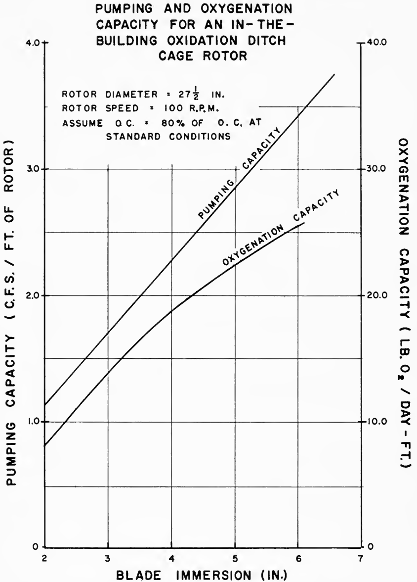
Typical oxygenation and pumping capacities of a cage rotor operating in a livestock oxidation ditch. The oxygenation capacity curve is 80 percent of the tested performance of the rotor in clean water corrected to standard temperature and pressure (Jones et al., 1969C). The pumping capacity curve was calculated using data reported by McKinney and Bella (1967). (Fig. 21)
