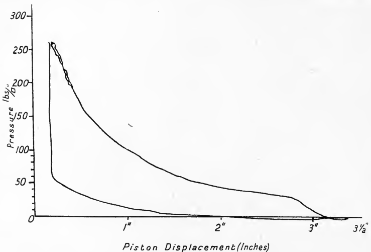
FIG. 52.—Indicator diagram of two-stroke engine. Mean pressure=62·81 lbs. per square inch. Speed of engine=900 r.p.m.
