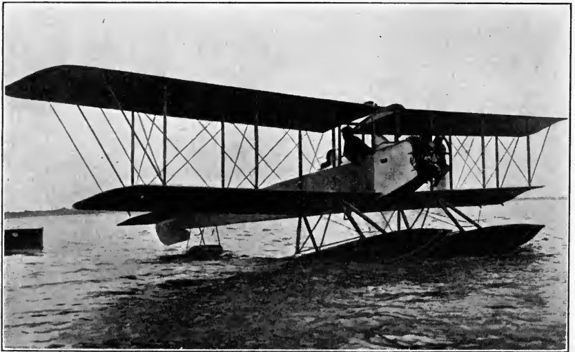
FIG. 19.—Sopwith 100 H.P. tractor hydro-aeroplane.
