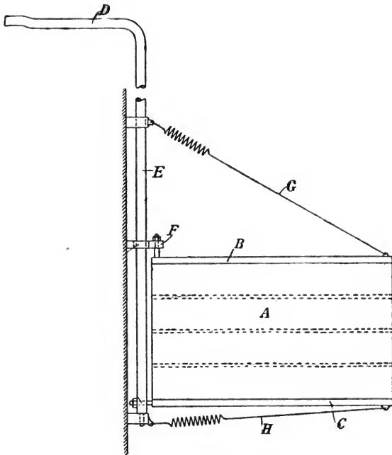
Fig. 47.—Shadbolt's Rudder.
