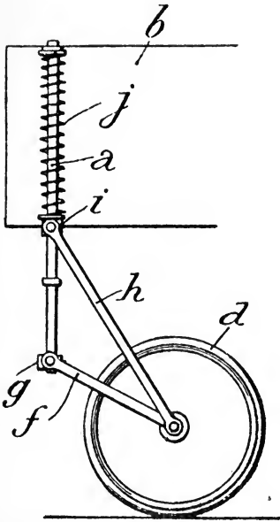
Fig. 62.—Blériot's Wheel Support.
