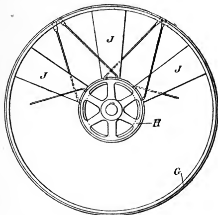
Fig. 10.—Lanchester's Propeller.
