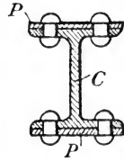
Fig. 46. — Esnault-Pelterie's Wing Beam.
