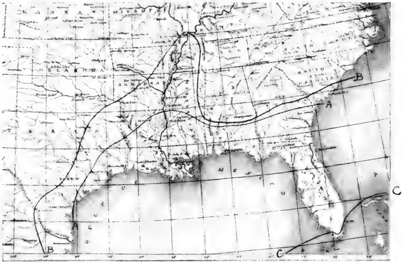
FIG. 1. Sketch map showing the approximate position of the shore line, A-A, at the beginning of the Wilcox transgression and B-B the area covered by the Wilcox sea during its maximum transgression. C-C, the extreme northern limit of the Wilcox flora under existing climatic conditions.
