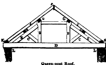
Queen-post Roof.
