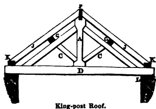
King-post Roof.
