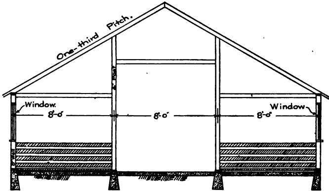
Fig. 288. Cross section of a hog house with gable roof.
