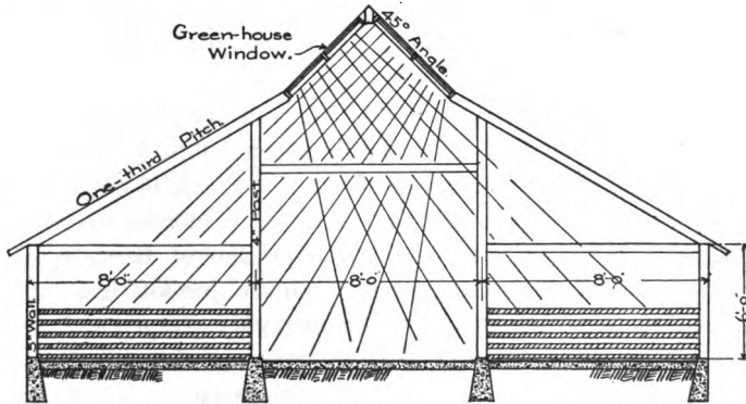
Fig. 289. Cross section of a hog house with a sky-light in the roof. Direct sunlight strikes all parts of the floor during the day.
