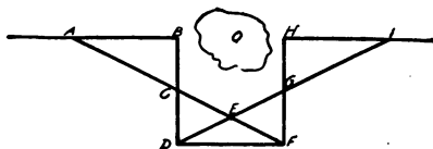
Fig. 10. Sketch showing method of extending a line beyond an obstacle.
