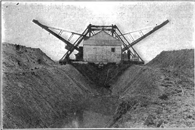
Fig. 67. An excavator for digging open ditches, which is carried on tracks laid at each side of the ditch.
