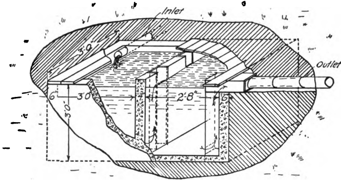
Fig. 308. A general view of a septic tank arranged to be connected with an underground irrigation or filter system without a siphon. (After Stewart.)
