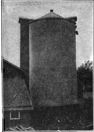
FIG. 295. A monolithic silo with concrete roof.
