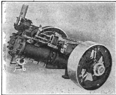
Fig. 237. The motor of an oil-burning tractor.
