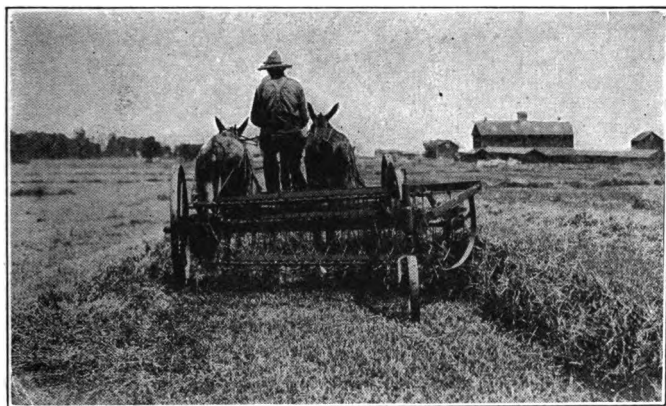
Fig. 166. A three-bar side-delivery rake at work.
