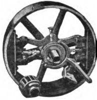
Fig. 238. One form of clutch. The wooden shoes are forced outward against the rim of the wheel, engaging it by friction.
