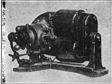
Fig. 232. A dynamo called the Auto-sparker.
