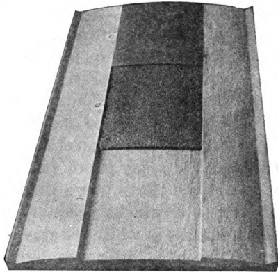
Fig. 83. Model of a gravel road illustrating the trench method of construction. A shows prepared sub-grade; B , first course of gravel; C , upper course of gravel. (Bul. 36, Office of Public Roads, U. S. Dept. of Agr.)
