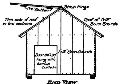
Fig. 265. End elevation of gable-roof colony hog house.
