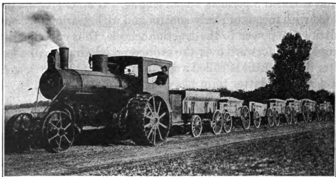
Fig. 251. An undermounted double-cylinder steam tractor.
