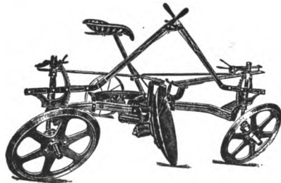
Fig. 117. A reversible disk plow. This plow is made to turn a right or left furrow by swinging the hitch from one end to the other.
