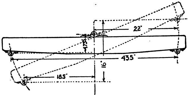
Fig. 214. A wagon doubletree illustrating the effect of not having the holes for the clevis pins in a straight line.
