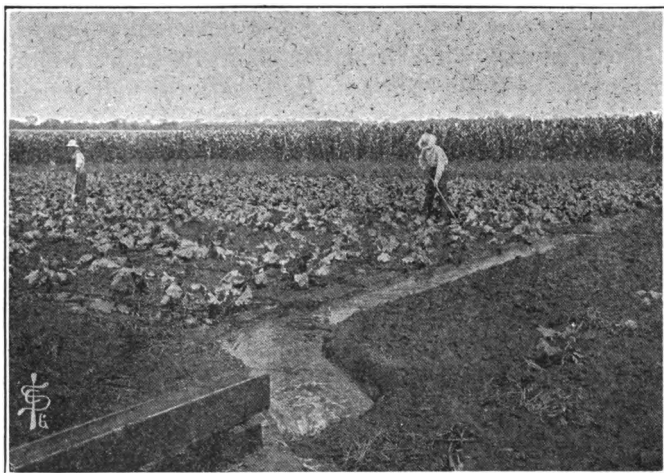
Fig. 78. Furrow irrigation with sewage water.
