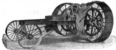
Fig. 239. The truck for a gas tractor, showing frame, gearing, and steering and driving wheels.
