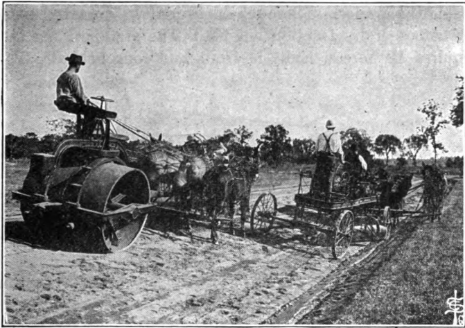
Fig. 91. A scraping grader and a horse roller at work.
