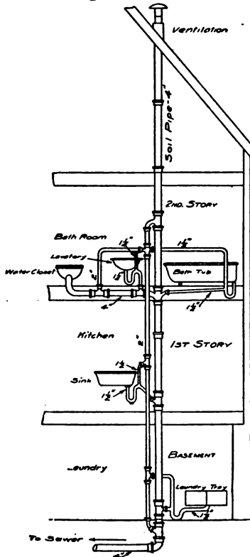
Fig. 307. A plumbing system for a two-story house. The vent pipe may be omitted with safety in country residences. (Mo. Eng. Exp. Sta. Bul.)
