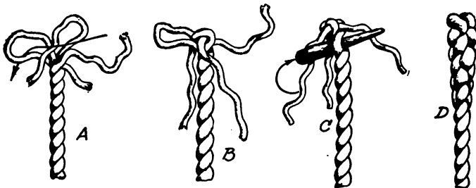
Fig. 338. Crowning.
