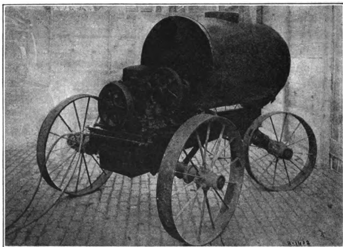
Fig. 193. A power sprayer.
