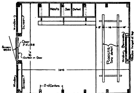
Fig. 271. Plan of an A-shaped colony poultry house. (Ia. Exp. Sta. Bul. 132.)
