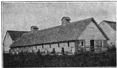
Fig. 270. A gable-roof hog house made of concrete blocks.
