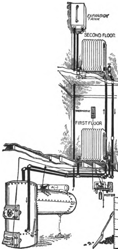
Fig. 220. A hot-water heating system. The locomotive type of furnace or boiler, although not in general use, is said to be quite satisfactory.
