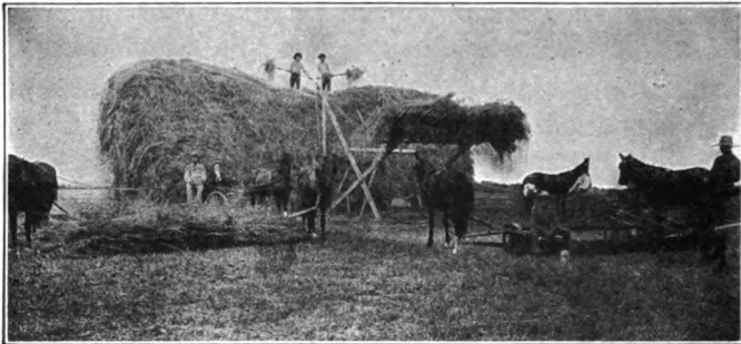
Fig. 169. A haying scene showing an over-shot stacker and sweep rakes at work.
