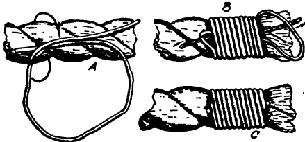
Fig. 337. Whipping.
