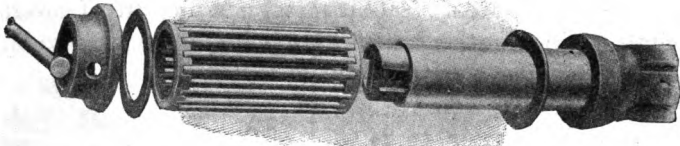
Fig. 103. A roller bearing for wagons. The hub of the wheel fits over the rollers shown.
