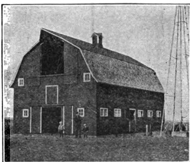
Fig. 285. A general farm barn with gambrel roof.
