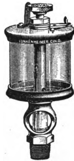
Fig. 106. A sight feed oil cup.
