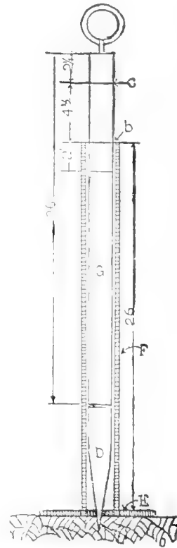
FIG. 5. Device for testing the compactness of the soil. (After C. A. Le Clair, in the Journal of Agricultural Research , Vol. V, No. 10.)
