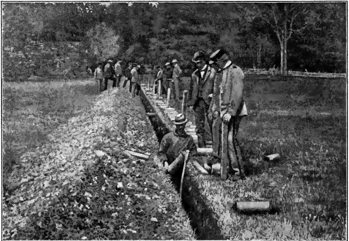
FIG. 9. LAYING A TILE DRAIN
