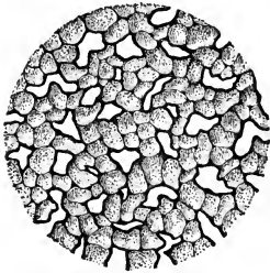
FIG. 6. AN ENLARGED VIEW OF A SECTION OF MOIST SOIL SHOWING AIR SPACES AND SOIL PARTICLES
