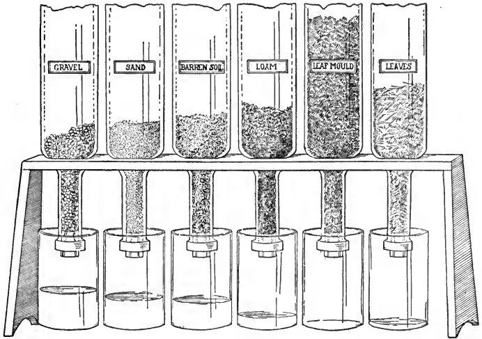
FIG. 7. APPARATUS FOR TESTING RETENTION OF WATER BY DIFFERENT SOILS
