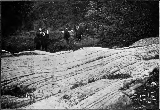
FIG. 1. ROCK MARKED BY THE SCRAPING OF A GLACIER OVER IT
