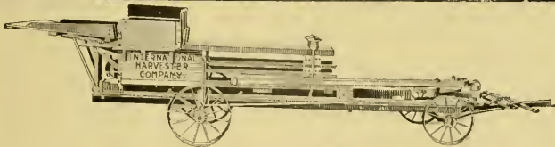
Two-Horse Pull Power Baling Press Ready for the Road
