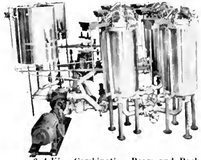
2 4-Kier Combination Beam and Package Dyeing Machines with Tandem Hookap
