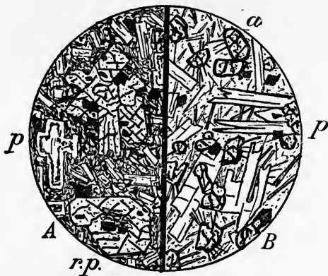
Fig. 36.— A , Pyroxene-Andesite (basaltic type). Kremnitz, Hungary. \times 14. p , Plagioclase. r.p. , Rhombic pyroxene (enstatite). Crystals of magnetite occur. Dark hemicrystalline groundmass. B , Glassy Pyroxene-Andesite (basaltic type). Dyke, Eskdale, Dumfries. \times 40. a , Granular augite, often set with radiating microlites from the glassy groundmass. p , Plagioclase in various stages of growth, often with characteristic bifurcating and incomplete terminations. Magnetite occurs. This rock exhibits the clear brown interstitial glass typical of many continental augite-andesites and "porphyrites."
