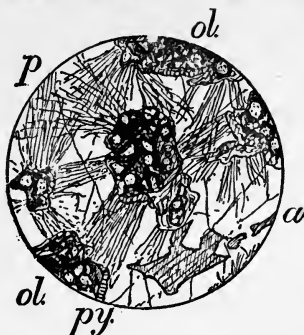
Fig. 31.—Gabbro rich in Olivine (Troctolite). Coverack, Cornwall. \times 12 . a , Irregular and very subordinate augite. ol , Olivine, altered, with development of serpentine and magnetite along the cracks. The surrounding felspars have become full of rifts which radiate from the decomposing olivine. p , Plagioclase (anorthite). py , Thin zones of pale brown pyroxene occasionally occurring on the margin of the olivine.
