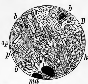
Fig. 27.—Altered Pyroxene-Mica-Diorite. Stanner Rock, Herefordshire. \times 12 . ap , Hexagonal and other sections of apatite included in the other minerals. b , Biotite. h , Green fibrous hornblende, occasionally in well marked crystals, developing at the expense of augite. ma , Magnetite. p , Plagioclase much altered. In the centre of the field is a pale crystal of original augite, with rectangular cleavage-cracks. Hornblende is developing in this by paramorphic change.
