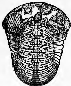
Fig. 114.— Stephanoceras modiolare (U. Jurassic). Viewed from the front, showing the broad section of the whorl, the shell having been broken away until a septum, with its folded surface, has become visible. The trace of the siphuncle is seen externally; and this example also illustrates the lack of connexion between the suture-lines and the surface-ornamentation.
