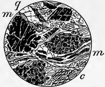
Fig. 23.—Crushed oolitic limestone passing into schist — Môtiers-en-Tarentaise, Alps of Savoy. \times 12 . c, Calcite. m, Mica in elongated and contorted folia. q, Quartz. Traces of oolitic structure remain in some of the limestone fragments; others are compact and almost opaque.
