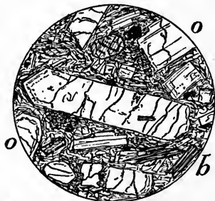
Fig. 33.—Trachyte, Ischia. \times 12 . b, Biotite. o, Orthoclase (sanidine) in fresh crystals, showing traces of zoning. Cleavages not distinct. Green soda-augite occurs; a cross-section lies near the top of the drawing. Fluidal hemicrystalline groundmass.
