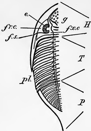
Fig. 127.—Trilobite ( Dalmania caudata ; Wenlock Beds). H , Head-shield; T , Body-segments; P , Pygidium. e , Eye. fx.c. , Fixed cheek. fr.c. , Free cheek. fs. , Facial suture (starting in this example from the lateral margin and finally passing round in front of the glabella). g , Glabella (bearing lateral furrows). pl. , Pleura.
