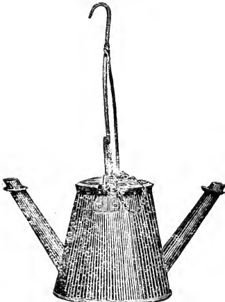
Wrought Iron Open Top Bucket Lamp, with Wire Bail and Chain attached to Cover.
