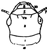
FIG. 601.—Head of Harpalus : a , dorsal aspect; b , ventral aspect; 1, occiput; 2 epicranium; 3, eye; 5, clypeus; 6, gula; 7, antenna; 8, labrum; 10, mandibles; 11 a , maxillary palpus; 11 f , galea or outer lobe of maxilla; 12 a , submentum; 12 b , labial palpus; cs , clypeal suture; gs , gular suture.
