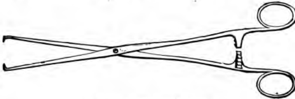
FIG. 9.—Luer's bullet-forceps.
