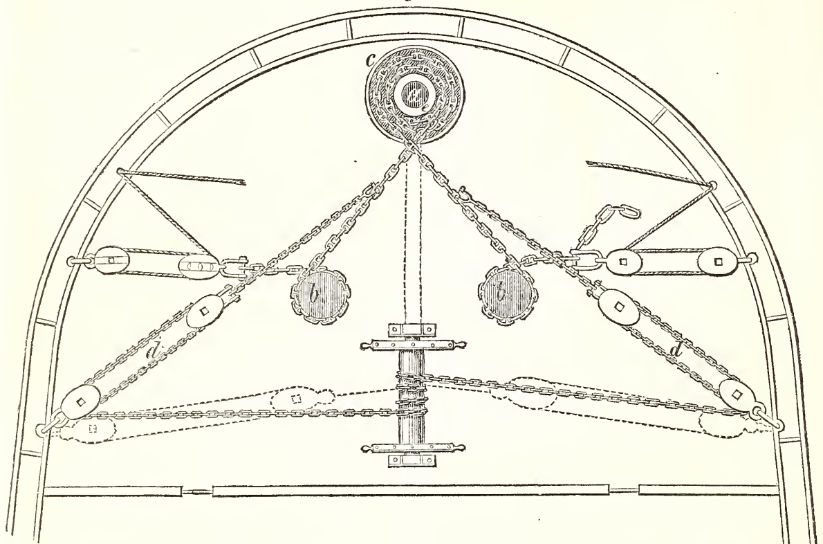
TEMPORARY STEERING APPARATUS OF THE GREAT EASTERN.
