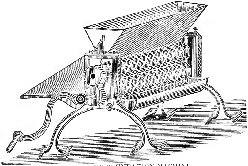
KING'S COMB-FOUNDATION MACHINE.
