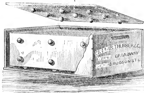
HOGES'S COMB-HONEY CARRIER.
