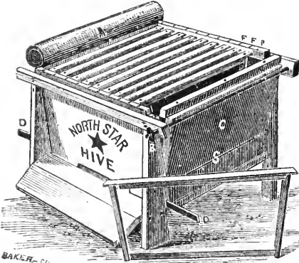
The above engraving shows the 1-inch second story of Hive No. 4, and contains 21 Prize Boxes and 7 Separators; each of the cases holding 3 prize boxes.
