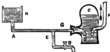
FIG. 2.—Whitehurst's Machine.
