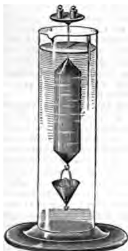
FIG. 1.—Nicholson's Hydrometer.
