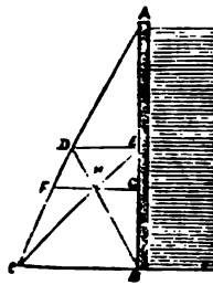
FIG. 5.—Centre of Pressure.
