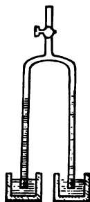
FIG. 4.—Hare's Hydrometer.
