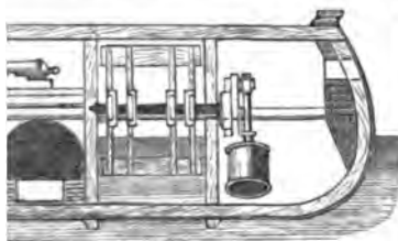
Fig. 2.—Demologos (section).
