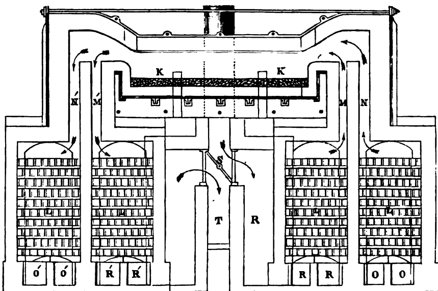
FIG. 5.—Siemens's Furnace.
