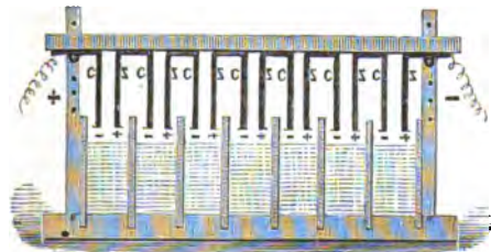
FIG. 4.—Modern Trough Battery.
