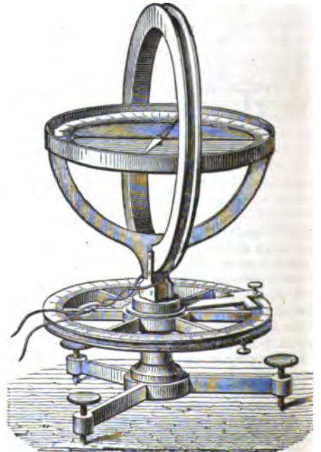
FIG. 19.—Sine Galvanometer.
