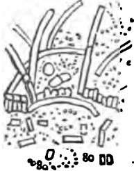
FIG. 7.— Arthrococcus , found in sour milk (Hallier).
